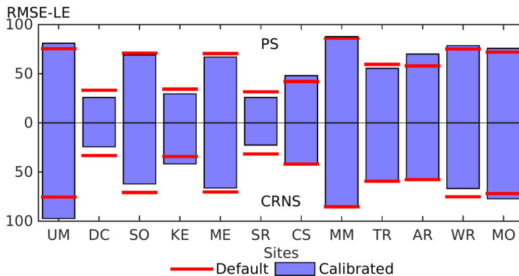
Figure A2.1: Root Mean Squared Error of simulated versus EC observed latent heat flux ( w m^{-2} ). The metric was computed over hourly day time data only. The upward bars represent PS-calibrated solutions, the downward bars represent CRNS-calibrated solutions. The Default runs are represented by the red horizontal lines, displayed twice for each site, to compare with both calibration strategies.
