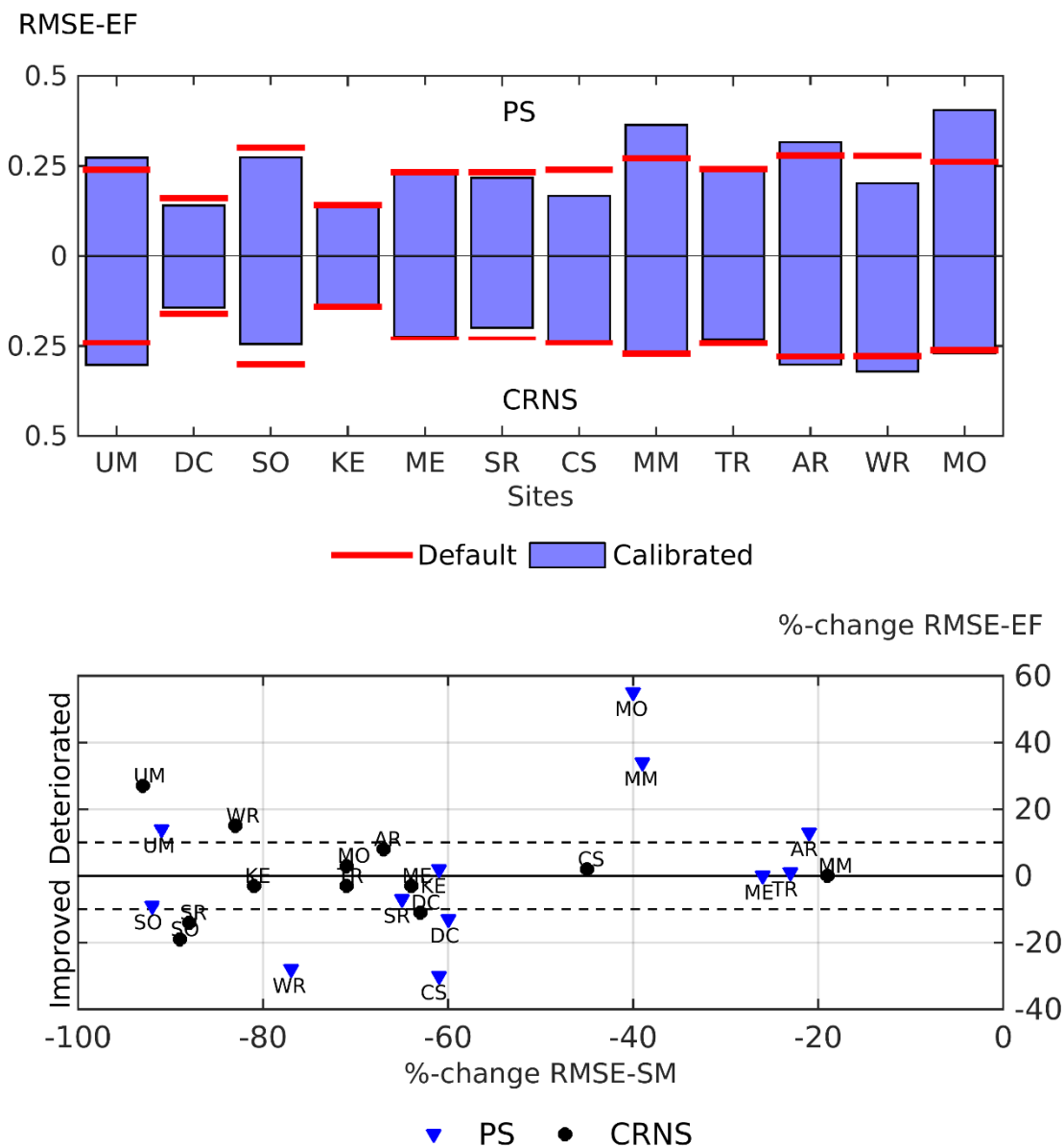
Figure 8: 8a) Root Mean Square Error (RMSE) values between observed and simulated Evaporative Fraction EF=LE/(LE+H) , per site, for default and calibrated (PS/CRNS) runs. 8b) Relative change in RMSE-EF and RMSE-SM after calibration plotted against each other.
