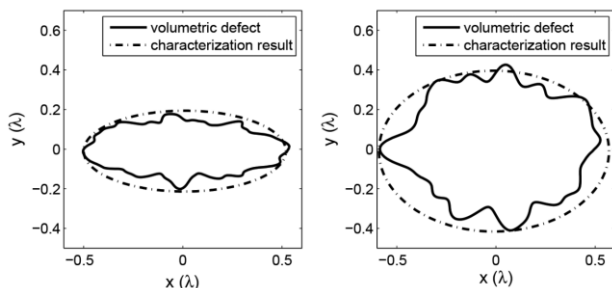
Figure 5: Accurate characterization of volumetric defects using a dynamic classifier approach.
