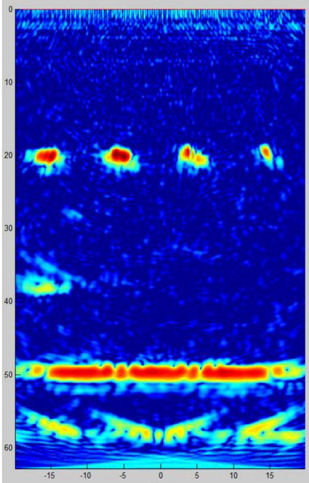
Figure 3: TFM image of stainless steel test specimen. Image shows 4 defects at 20mm depth and the back face of the specimen at 50mm.
