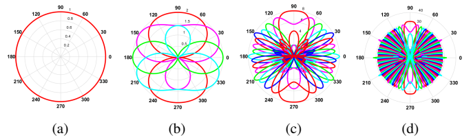
Fig. 4: Beam patterns created using Equation 1 with (a) M = 1 and K = 1 , (b) M = 2 and K = 4 , (c) M = 8 and K = 16 and (d) M = 32 and K = 64 at both the transmitter and receiver
