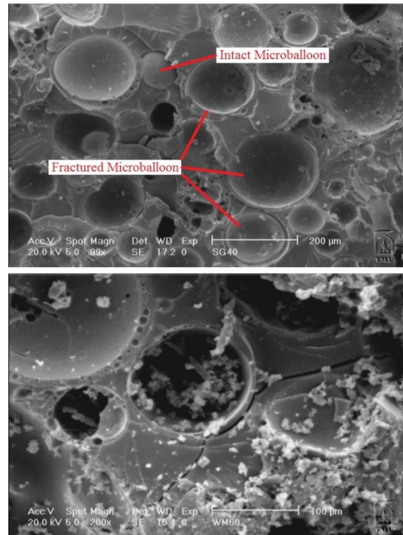
Figure 5. Crack paths through microballoon, matrix and interfacial surfaces between them in SEM figures from fractured surfaces
