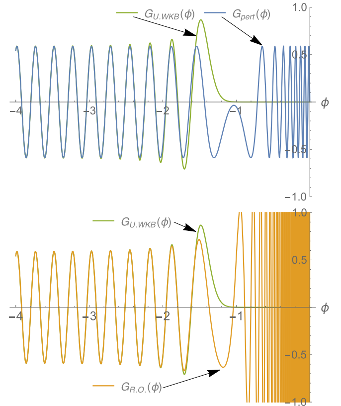
FIG. 5. Comparison of the U.WKB, perturbative (top panel) and RO (bottom panel) wavefunctions, for the example of Fig. 2, which corresponds to the expansion parameter of the perturbative and RO approaches being \epsilon = \pm 1/50 . The RO wavefunction more closely tracks the U.WKB wavefunction as we approach the turning point, but the difference is small. Under the barrier, neither the perturbative nor RO wavefunctions fall off as expected. This is consistent with those approximations begin essentially high-energy.
