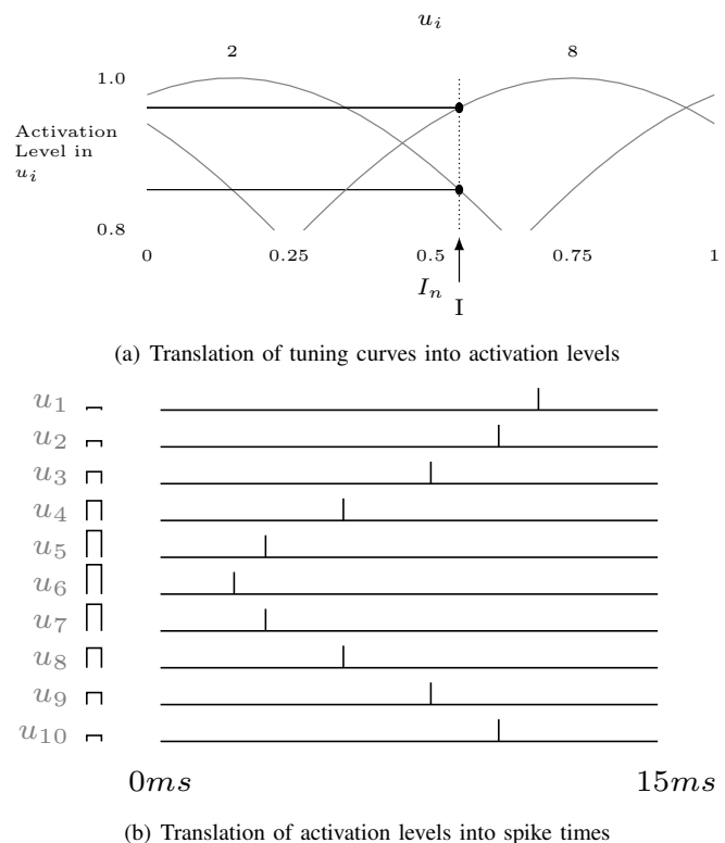
Fig. 2. Generation of a temporal sequence from a value in an input dimension and a bank of neurons tuned to points within that dimension. (a) shows the generation of an activation value for each neuron ( u_i ) from within the bank of input neurons representing input dimension ( I_n ). An example input value, at arrow I , of 0.55 is shown by the vertical dotted line. Activation values are established by the vertical point at which this dotted line crosses the tuning curve for a ( u_i ) neuron. Example tuning curves are shown for neurons 2 and 8, tuned to values of 0.15 and 0.75 respectively. The vertical locations of the horizontal lines from this curve then represent the activation levels. (b) demonstrates the type of output firing sequence that results. The height of the bars shown next to each u_i represents the activation level generated from the intersection of a given input value and the neuron's tuning curve.
