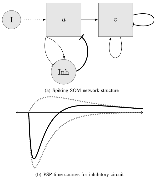
Fig. 1. (a) Spiking SOM network structure: an actual input value I is encoded into spikes times by nodes in layer u ; the inhibitory unit causes oscillations, allowing continuous input to be presented to u (see section II-C1 for details); feedforward connections from u to v drive firing in v ; early firing in v determines the location of output activity in v through lateral (neighbourhood) connections (see section II-C2 for details). (b) shows the time course of the post-synaptic potential from both of the u to Inh synapses (inhibitory is the lower dotted line, excitatory is the upper dotted line), together with the combined effect on the membrane potential of Inh_u (solid line)
