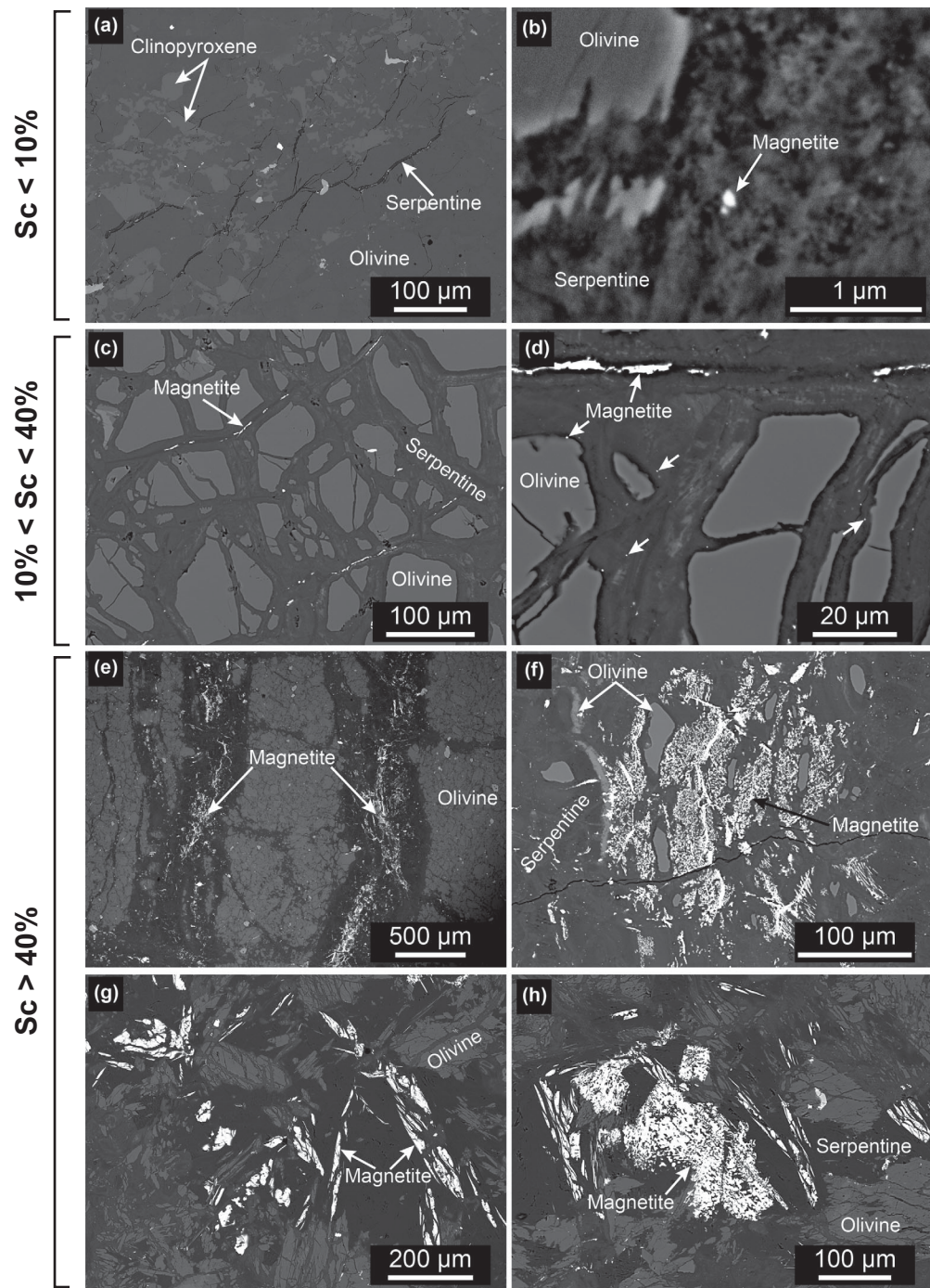
Figure 3. BSE images of serpentinized peridotites from the Mirdita OCC. The range of serpentinization degree of each group of images is shown. (a and b) Magnetite grains in samples with a very low serpentinization degree (2%) are predominantly (sub)micron in size; occasionally larger grain aggregates (5–10 μm) occur. (c and d) Magnetite grains in samples with an intermediate serpentinization degree (10% < Sc < 40%) are again mainly (sub)micron sized. However, larger grains frequently develop in the center of serpentine veins (Type 2 veins). (e–h) Samples characterized by high degrees serpentinization (>40%) display large (>50 μm), complex structured magnetite grains either (e and f) making up major parts within wide serpentine vein centers, or (g and h) heterogeneously distributed throughout the rock.
