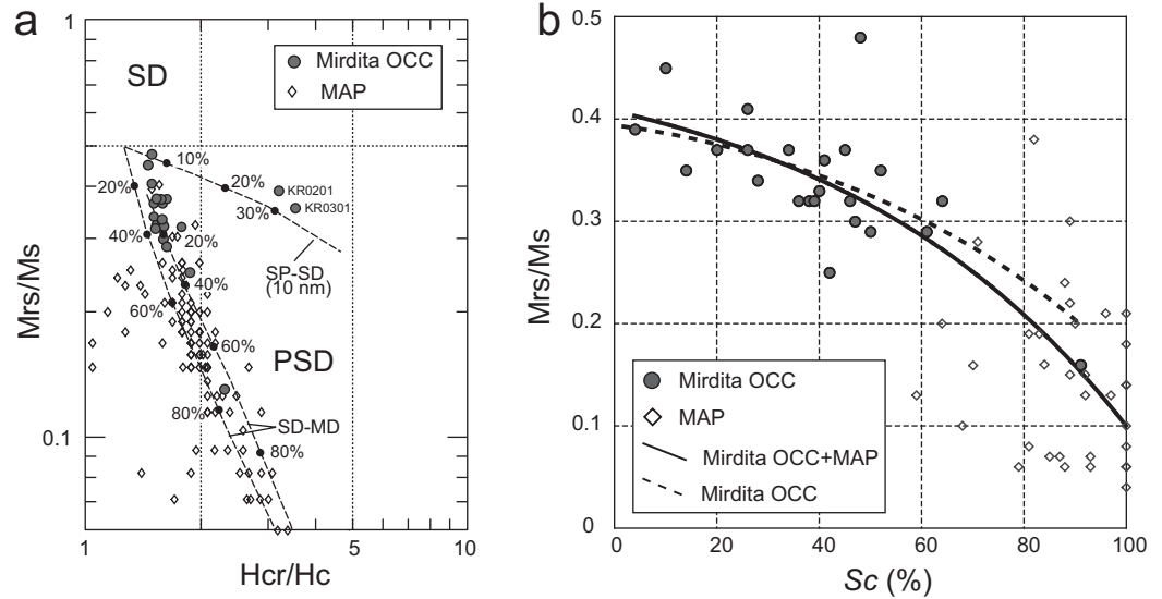
Figure 7. (a) Day plot [Day et al., 1977] for 21 representative samples from the Mirdita OCC and MAP (see text). Most of the samples follow the theoretical mixing curves SD-MD for magnetite (dashed lines) of Dunlop [2002], showing a variable proportion of MD particles from <10% up to ~80%. Two samples are aligned along the SD-SP mixing curve and contain up to 30% SP grains. (b) Remanence ratio (Mrs/Ms) against the degree of serpentinization (Sc) for the same combined data set. Both best-fit curves for the Mirdita OCC (dotted line) and combined data sets (full line) are described by second-order polynomial functions.
