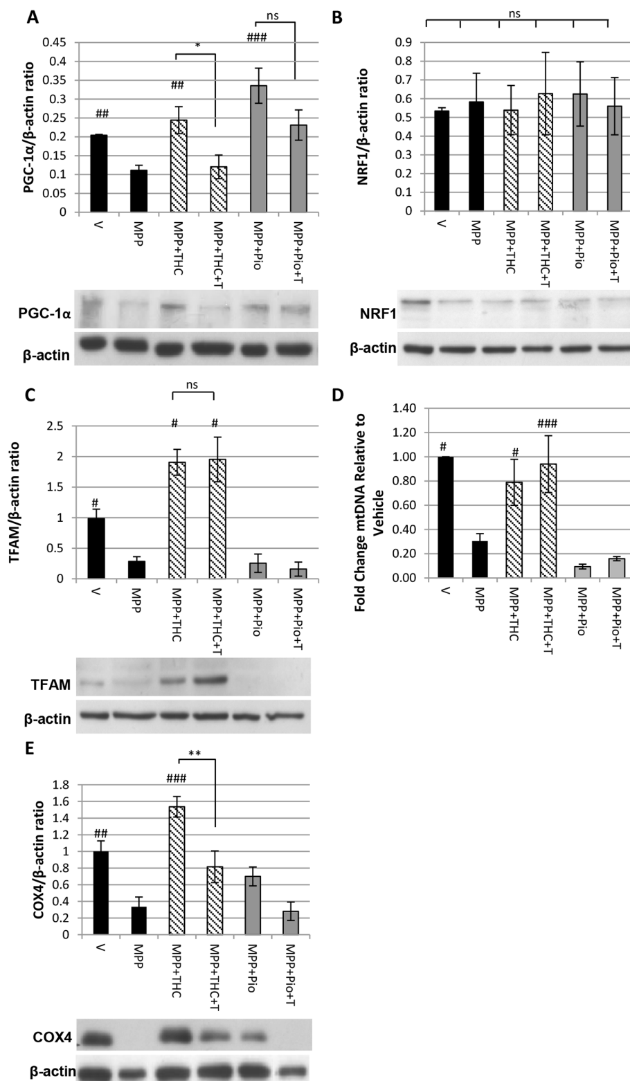
Figure 2: \Delta^9 -THC but not pioglitazone induces mitochondrial biogenesis. Western blot showing the effect of MPP + , \Delta^9 -THC, pioglitazone (pio) and T0070907 (T) on A . PGC-1 \alpha expression (n = 5, one-way ANOVA with Scheffe post-hoc test), B . NRF1 expression (n = 5, one-way ANOVA with Tukey HSD post-hoc test) and C . TFAM expression (n = 3, one-way ANOVA with Tukey HSD post-hoc test). D . QPCR on genomic DNA extracts to determine the ratio between mitochondrial and genomic DNA. Cells were treated with MPP + , \Delta^9 -THC, pioglitazone (pio) and T0070907 (T) (n = 3, one-way ANOVA with Tukey HSD post-hoc test). E . Western blot showing the effect of MPP + , \Delta^9 -THC, pioglitazone (pio) and T0070907 (T) on COX4 expression (n = 4, one-way ANOVA with Tukey HSD post-hoc test). Protein data were corrected to \beta -actin levels which served as loading control. Each bar represents the mean \pm SEM (#p<0.05, ##p<0.01, ###p<0.0001 vs. MPP + ).
