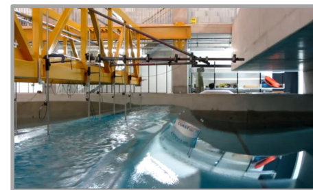
The X-MED buoy moored in the Ocean Basin: being hit by a wave (left) and showing the retroreflective markers used for 3D motion tracking (right).
