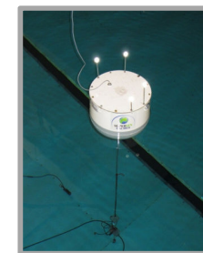
The X-MED buoy moored in the Ocean Basin: being hit by a wave (left) and showing the retroreflective markers used for 3D motion tracking (right).
