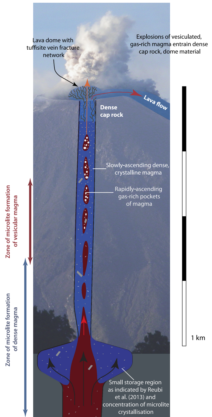
Fig. 9. Conceptual model of shallow processes occurring at Volcán de Colima. Blue portions represent the dense, slowly ascending magma and red, the vesicular, gas-rich and fast ascending magma. Explosions lead to open-system degassing and increased extrusion of dome and lava flows, degassing emissions are shut off as the conduit becomes sealed by the formation of tuffsite veins. The horizontal axis is slightly exaggerated, the crater is 250 m across for reference. (For interpretation of the references to colour in this figure legend, the reader is referred to the web version of this article.)
