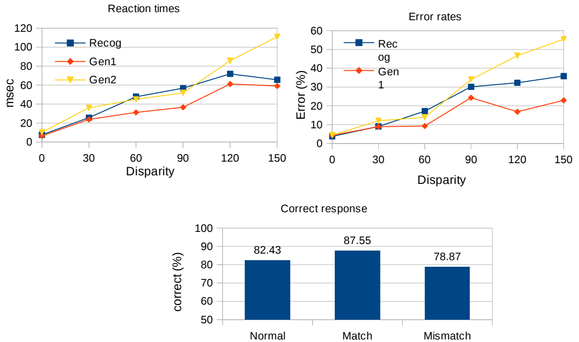
Figure 6.11 Comparison of the results when the model receives congruent or incongruent proprioception in the case of the Gen1 image dataset.
