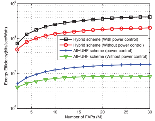
Figure 4. Energy Efficiency of a hybrid HetNet and all-UHF HetNet with and without power control with varying number of FAPs for N=100 and F=5 .
