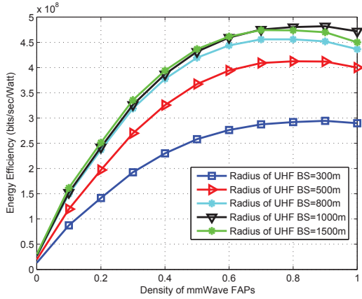
Figure 6. Energy Efficiency of a hybrid HetNet with power control with varying density of mmWave FAPs for M=15 , F=5 and N=100 .
