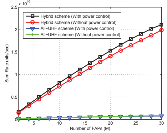
Figure 3. Sum-rate of a hybrid HetNet and all-UHF HetNet with and without power control with varying number of FAPs for N=100 and F=5 .
