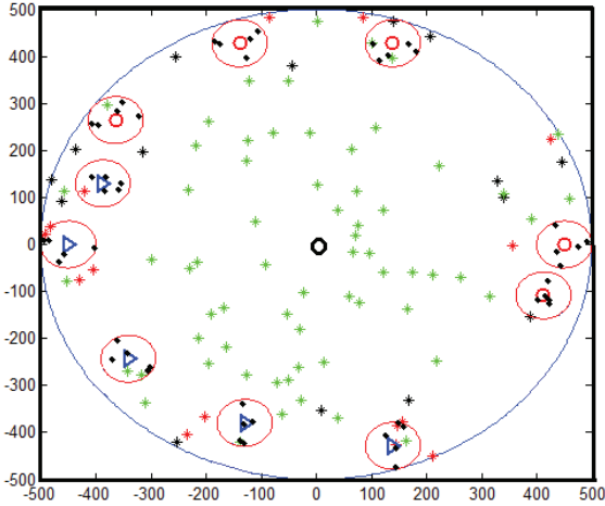
Figure 2. Snapshot of the HetNet with blue triangles showing UHF FAPs and red circles showing mmWave FAPs. Green stars representing the MUEs connected to MBS, red stars representing the MUEs connected to FAPs and black stars representing the MUEs in outage ( M=10 , N=100 and F=5 ).
