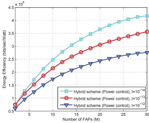
Figure 5. Energy Efficiency of a hybrid HetNet with power control for various interference threshold with varying number of FAPs for N=100 and F=5 .
