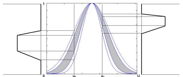
Fig. 5. Construction of T2FSs from IVFSs
