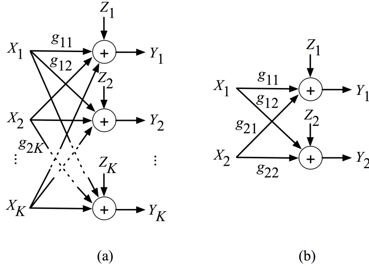
Fig. 1: (a) The K -user Gaussian Interference Channel (G-IC) (b) The 2-user G-IC.
