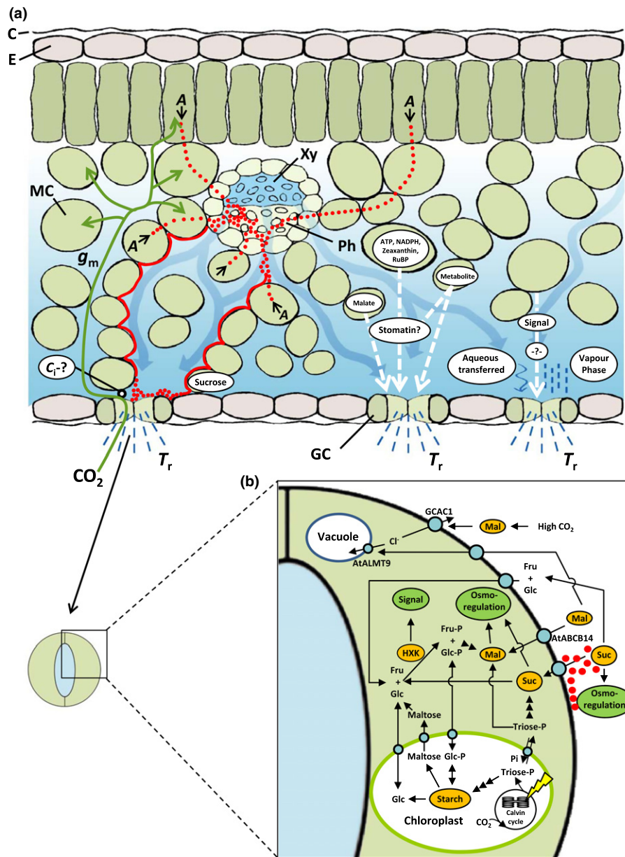
Fig. 1 Schematic diagram of a leaf cross-section showing possible mechanisms that connect mesophyll and guard cells and affect stomatal behaviour (a). \text{CO}_2 absorbed from the atmosphere through the stomatal pore diffuses towards the mesophyll cells (green line), where it is used for photosynthesis (A). Sucrose (Suc, represented by red dots) moves from the mesophyll cells (MC) toward the phloem (Ph). Water (blue arrows) coming out of the xylem (Xy) move toward the guard cells and evaporate ( T_r ) to the atmosphere. Some of the apoplastic Suc (red line) is carried by the transpiration stream toward the guard cells (GC) and accumulates at the GC. The diagram includes additional potential effectors (such as \text{C}_i , metabolites and aqueous- vs vapour-carried signals). (b) Schematic diagram of the primary metabolism in GC and the potential effects. Suc may accumulate at the GC cell wall (red dots), and may have an extracellular osmotic effect. Suc may enter the GC via Suc transporters or might be cleaved in the apoplast into glucose (Glc) and fructose (Fru) that also enter GC via a hexose specific transporter. In the cytosol, Suc may have an osmotic effect. Photosynthesis in GC yields triose-phosphates (triose-P) which may be converted to starch within the chloroplast or exported to the cytoplasm, where it might be converted to Suc or malate. Starch degradation may also contribute to Suc and malate accumulation. Malate may be produced in guard cells and/or arrive from mesophyll cells and enter the guard cells through malate transporters such as AtABC14. Within guard cells malate may activate vacuolar \text{Cl}^- transporters such as AtALMT9, contributing to stomatal osmolarity and opening. High \text{CO}_2 concentration may increase concentrations of malate produced in the mesophyll stimulating anion efflux through channels such as GCAG1 and close stomata. The cytosolic Glc and Fru obtained from Suc cleavage or from starch degradation must be phosphorylated into Glc-P and Fru-P to be further metabolized. Sensing of Glc and Fru by hexokinases (HXK) may generate a signal that closes stomata. C, cuticle; E, epidermis; MC, mesophyll cell; GC, guard cell; A, photosynthesis; Xy, xylem; Ph, phloem; g_m , mesophyll conductance to \text{CO}_2 ; \text{C}_i , substomatal \text{CO}_2 concentration; T_r , transpiration; ATP, adenosine triphosphate; NADPH, nicotinamide adenine dinucleotide phosphate; RuBP, ribulose 1, 5-bisphosphate; Glc-P, glucose phosphate; HXK, hexokinase; Suc, sucrose; Triose-P, triose phosphate. White circles and white arrows, mesophyll-driven signals affecting stomatal movement; red dots and lines, sucrose paths; blue faded arrows, the flow of water from xylem toward the stomata; green arrow, \text{CO}_2 movement; blue circles, transporters; green circles, the effect on stomatal aperture.
