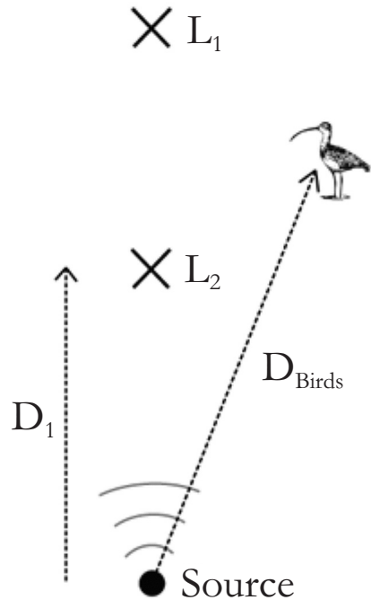
Figure 1. Placement of sound recording instruments ( X L_1 and X L_2 ) relative to the source of the sound. By using sound levels recorded at a known distance (e.g. D_1 ) to calculate the power of the source it is possible to determine approximately the decibel (dB(A)) level experienced at other distances ( D_{\text{Birds}} ).
