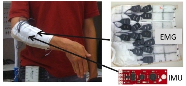
Figure 2. JPL BioSleeve mounted on the forearm, with EMG and IMU sensors.
