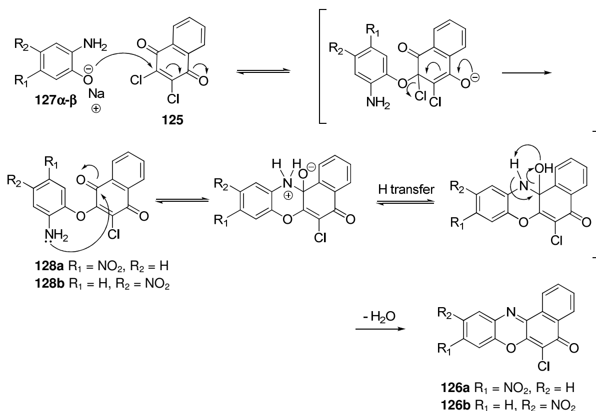
Scheme 1.41: Suggested mechanism for the formation of nitro-6-chlorobenzo[ a ]phenoxazin-5-one (1980JOC2155).
