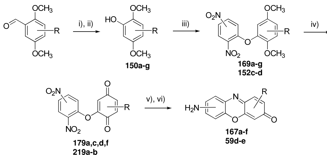
Scheme 4.4: Recapitulative synthesis of phenoxazinones 167a-f and 59d-e
