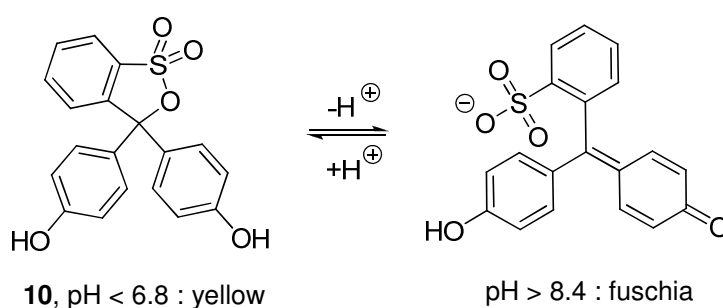
Scheme 1.3: Acidic and basic forms of phenol red.
