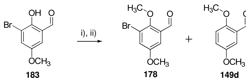
Scheme 2.12: Protection of 2-hydroxy-5-methoxybenzaldehyde 183
