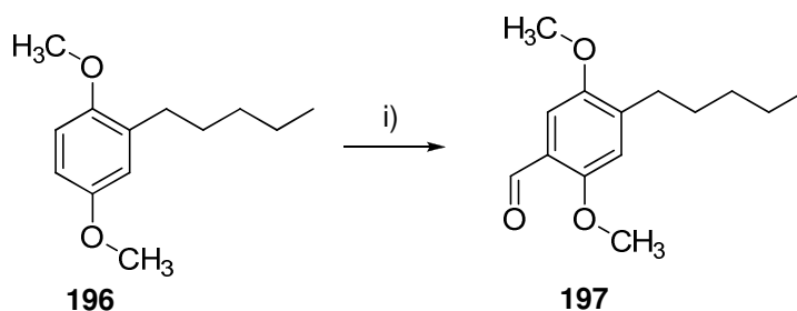
Scheme 2.18: Formylation of 1,4-dimethoxy-2-pentylbenzene 196 i) TFA, urotropine, reflux, 82.4%.
