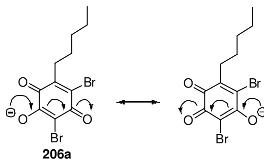
Scheme 2.28: Stabilisation of 3,5-dibromo-3-hydroxylate-6-pentylbenzoquinone anion 206a .
