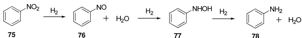
Scheme 1.23: Suggested enzymatic reduction pathway of nitro compounds (1954BCJ42).
