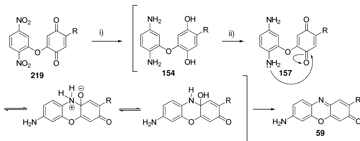
Scheme 2.49: Possible mechanism of formation of 7-aminophenoxazin-3-ones 59 i) MeOH, Pd/C 5%, H 2 , P = 2.4bar, ii) Ag 2 O, MeOH.
