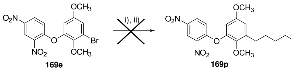
Scheme 2.32: Attempted preparation of 2,4-dinitro-2',5'-dimethoxy-3'-pentyldiphenylether 169p
