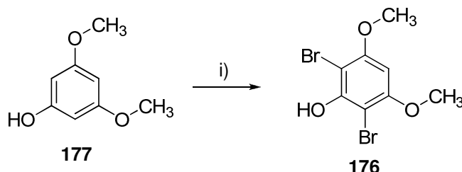
Scheme 2.21: Bromination of 3,5-dimethoxyphenol 177 i) Br 2 , DCM, 72.6%.
