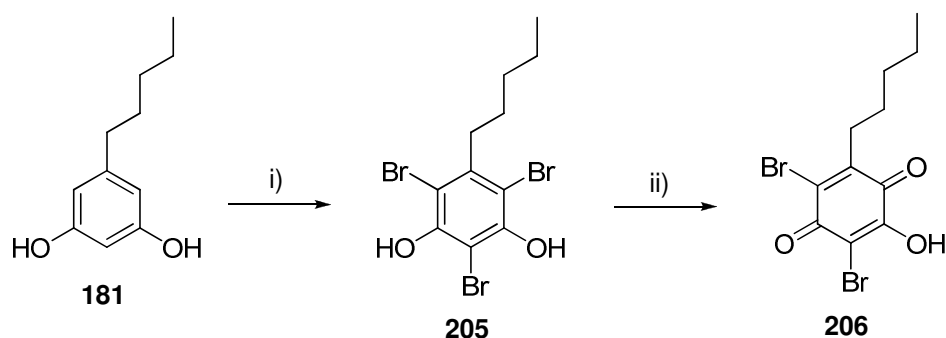
Scheme 2.24: Preparation of 2,6-dibromo-3-hydroxy-5-pentyl-1,4-benzoquinone 206 i) Br_2 , AcOH, NaOAc, 0^\circ C to R.T., 5h, 92.2%; ii) Fremy's salt, K_2HPO_4 , H_2O , CH_3CN , R.T., 81.6%.
