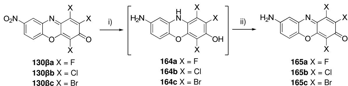
Scheme 2.5: Preparation of 8-amino-1,2,4-trihalogeno-3 H -phenoxazin-3-one 165a-c i) H 2 , Pd/5%C or PtO 2 , MeOH/EtOAc; ii) AgO or Ag 2 O or MnO 2 , MeOH; 165a : 98.0%; 165b : 97.6%, 165c : 94.8%.
