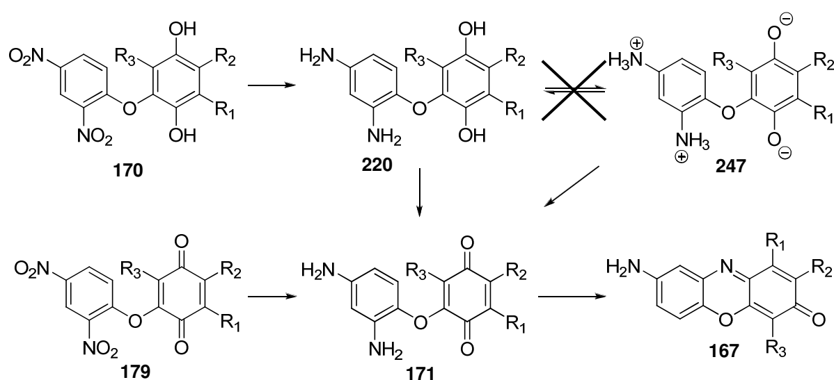
Scheme 4.5: Relation between the evidenced intermediates and their role in the cyclisation of 8-aminophenoxazin-3-one 167 .
