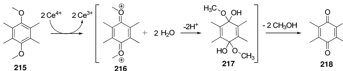
Scheme 2.37: Suggested intermediates for the formation of duroquinone via CAN oxidation of 1,4-dimethoxybenzene-2,3,5,6-tetramethylbenzene 215 (1976JOC3627).
