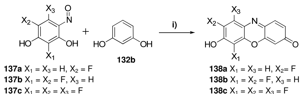
Scheme 1.45: Condensation of fluorinated 4-nitrosoresorcinol 137a-c and resorcinol 132b i) conc. H_2SO_4 , EtOH, \Delta = 80^\circ C ; 138a , 16.7%; 138b , 41.3%; 138c , 48.5% (2008USP7432372).
