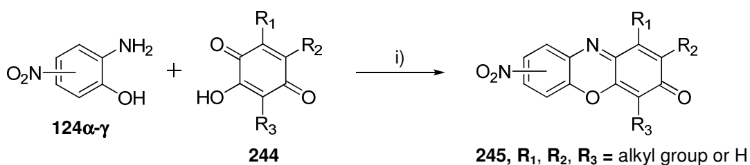
Scheme 4.2: Possible preparation of nitroalkylphenoxazin-3-ones 245
