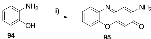
Scheme 1.30: Oxidative condensation of o -aminophenol i) FeCl 3 or K 2 Cr 2 O 7 , CH 3 COOH; yield not given (1890MI2792).
