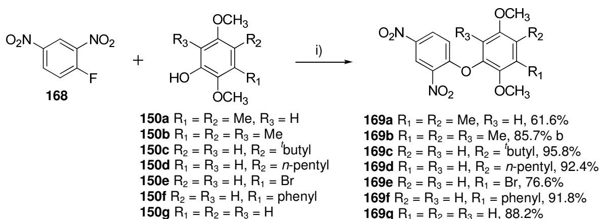
Scheme 2.25: Preparation of 2,4-dinitro-2',5'-dimethoxydiphenylether 169a-g
