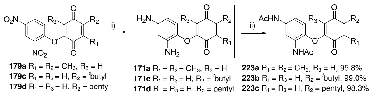
Scheme 2.44: Trapping of the 2,4-aminophenoxy-2',5'-benzoquinones intermediates via acetylation i) MeOH, Pd/C 5%, \text{H}_2 , P = 2.4\text{bar} ; ii) Acetic anhydride.
