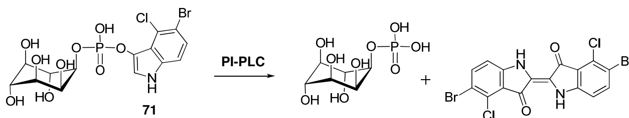
Scheme 1.19: PI-PLC hydrolysis of 5-bromo-4-chloro-3-indoxyl- myo -inositol-1-phosphate 71 .
