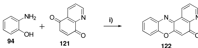
Scheme 1.38: Preparation of 5 H -pyrido[3,4 a ]phenoxazin-5-one 122
