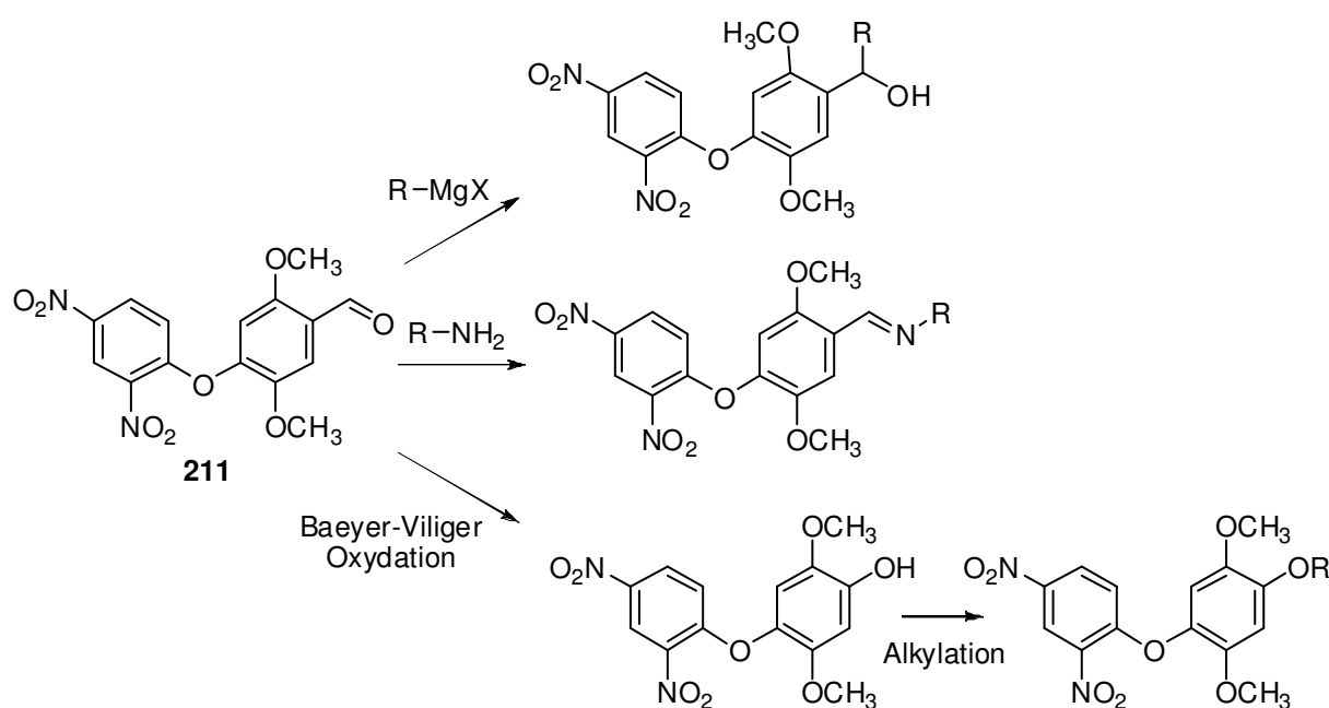
Scheme 4.8: Example of possibly interesting derivatization of 2,4-dinitro-2',5'-dimethoxy-3'-carbaldehydediphenylether 211 .
