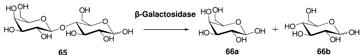
Scheme 1.17: Lactose hydrolysed into \beta -D-galactose and \alpha/\beta -D-glucose.
