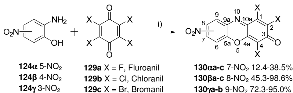
Scheme 2.1: Preparation of nitro-1,2,4-trihalogeno-3 H -phenoxazin-3-ones i) EtOH, NaOAc, R.T.
