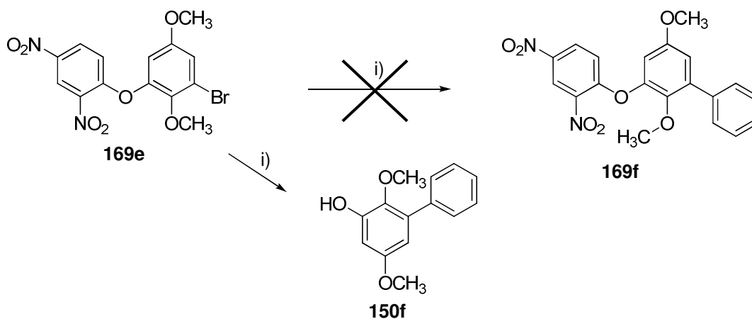
Scheme 2.33: Suzuki coupling of 2,4-dinitro-3'-bromo-2',5'-dimethoxydiphenylether 169e
