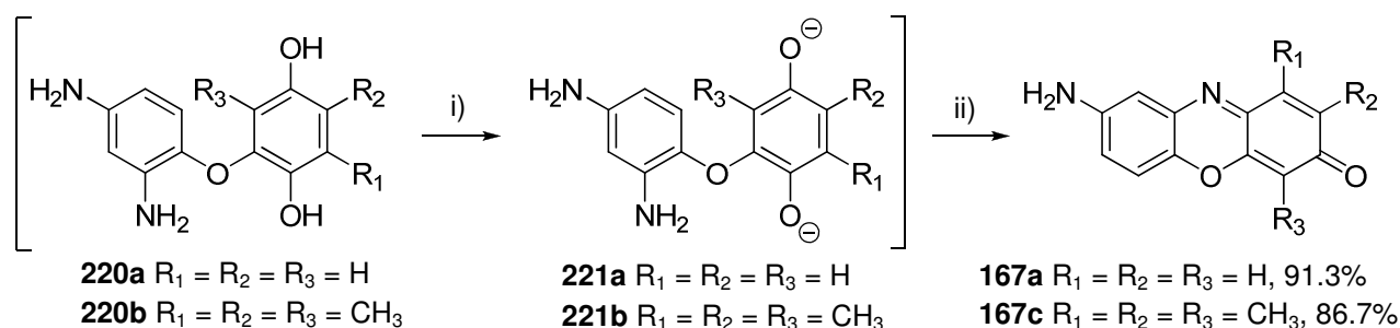
Scheme 2.40: Oxidative cyclisation of 2,4-diamino-2',5'-dihydroxydiphenylether derivatives
