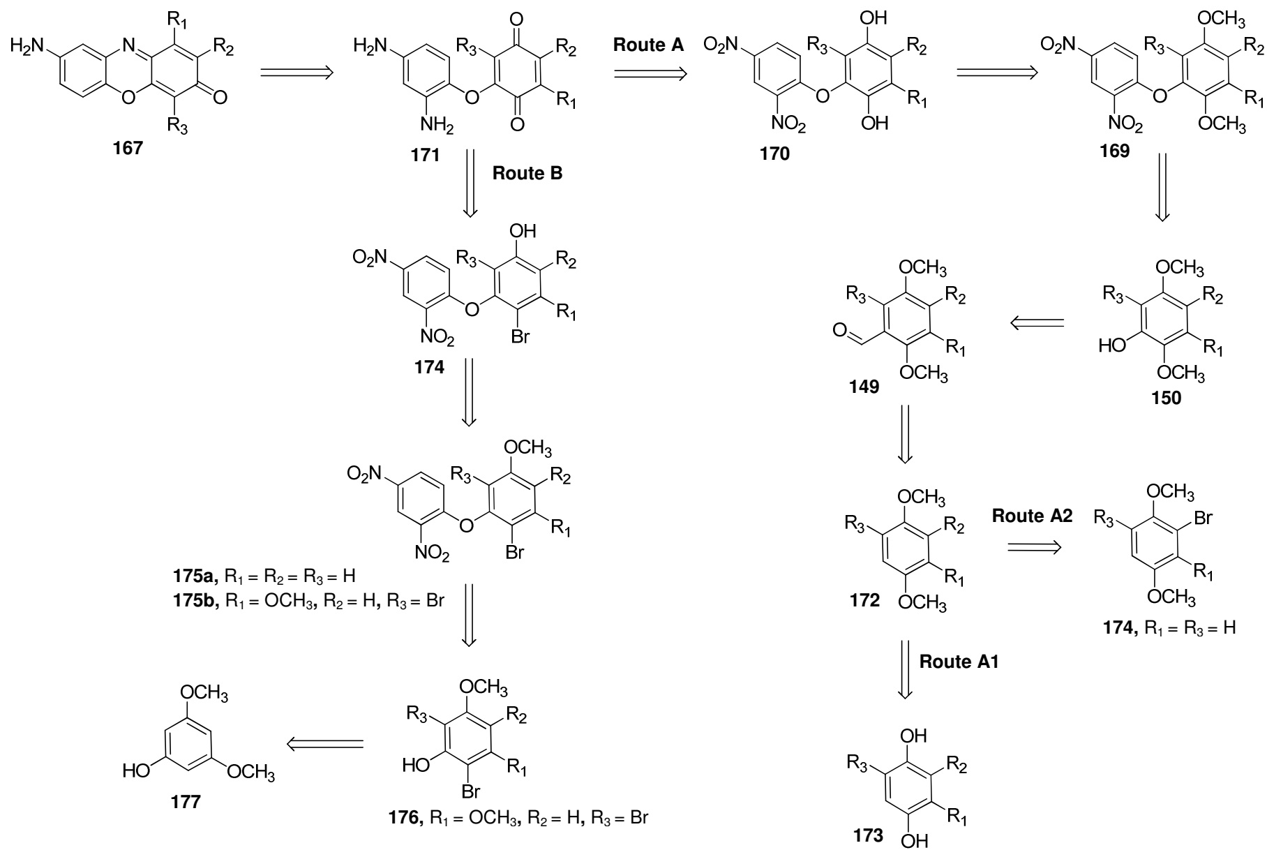
Scheme 2.8: Retrosynthetic analysis on potential 8-amino-phenoxazin-3-ones derivatives.
