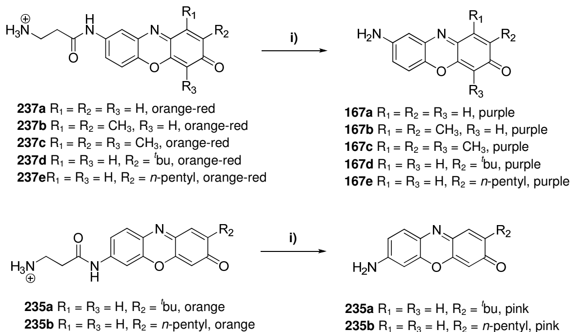
Scheme 3.5: Expected reaction upon enzymatic hydrolysis of substrates 237a-f and 235a-b i) \beta -alanine aminopeptidase
