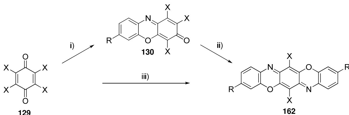
Scheme 2.3: Formation of triphenodioxazinone 162
