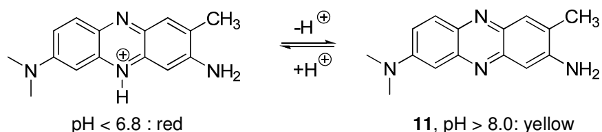
Scheme 1.4: Acidic and basic forms of neutral red.
