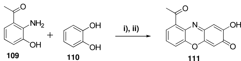
Scheme 1.33: Synthesis of 2-hydroxy-1-acetylphenoxazin-3-one i) K_3(FeCN_6) , AcOH; ii) H_2O ; 43% (1957LA72).
