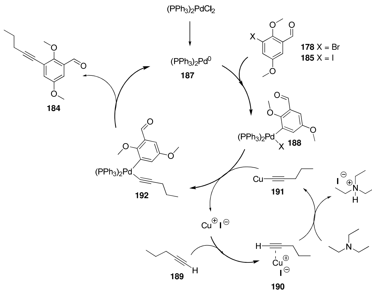
Scheme 2.15: Hypothetic catalytic cycle of the Sonogashira cross-coupling reaction.
