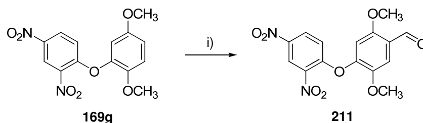
Scheme 2.34: Formylation of 2,4-dinitro-2',5'-dimethoxydiphenylether 169g
