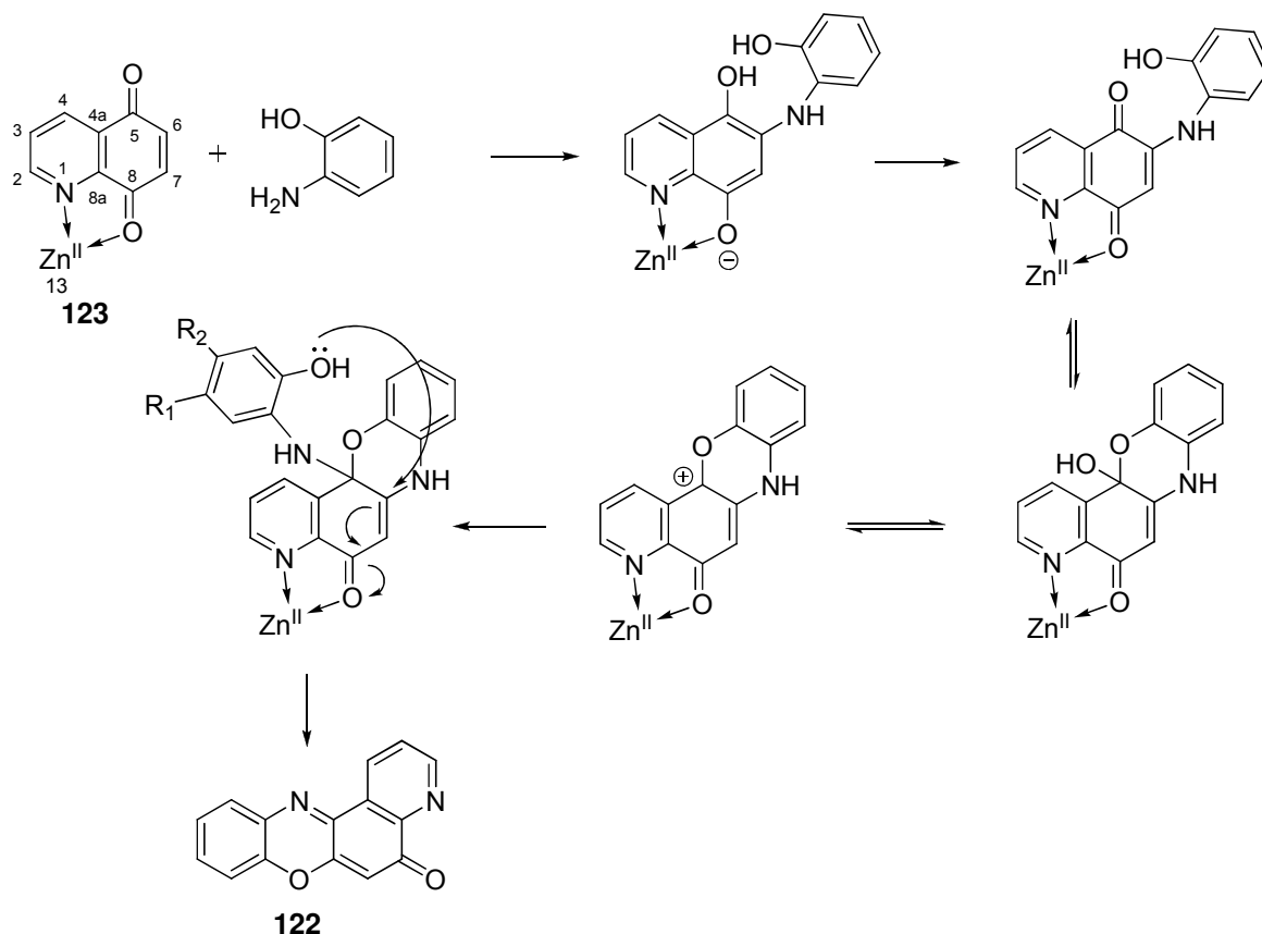
Scheme 1.39: Suggested mechanism for the formation of 5 H -pyrido[3,4- a ]phenoxazin-5-one (2002JME5205)
