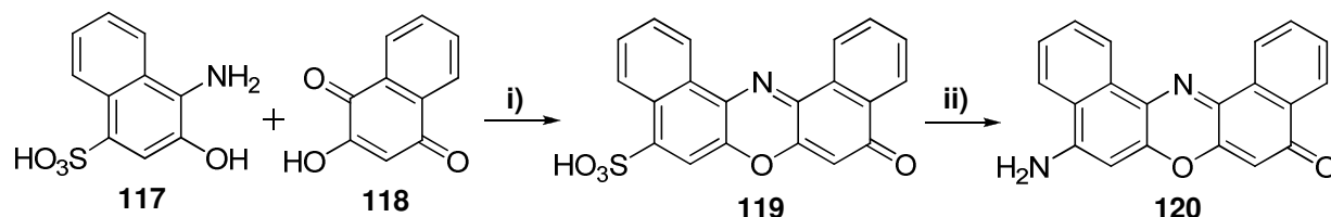
Scheme 1.37: Preparation of aminodinaphthoxazone 119
