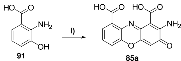
Scheme 1.31: Oxidative condensation of 3-hydroxyanthranilic acid 91 i) MnO 2 , 92% (1978CA22792d).
