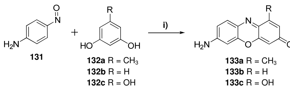
Scheme 1.43: Condensation of p -nitrosoaniline and resorcinol derivatives i) conc. HCl, EtOH, reflux; 133a , 1.5%; 133b , 14.8%; 133c , yield not given (1969M1670).
