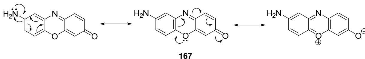
Scheme 2.56: Electron conjugation within 8-amino-3 H -phenoxazin-3-one.
