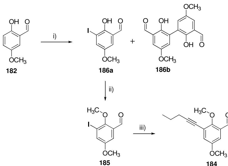
Scheme 2.14: Preparation of 2,5-dimethoxy-3-iodobenzaldehyde 185
