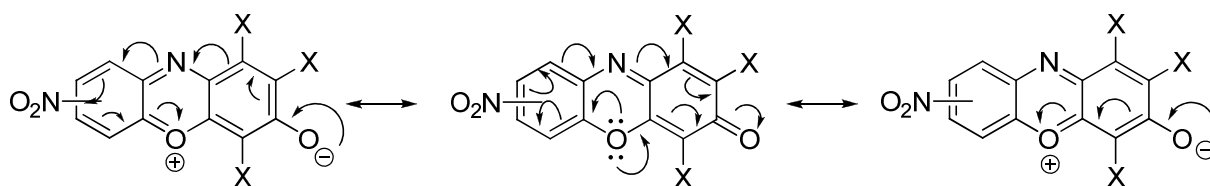
Scheme 2.2: Electron conjugations within the phenoxazin-3-one core responsible for the weakening of the C=O bond.
