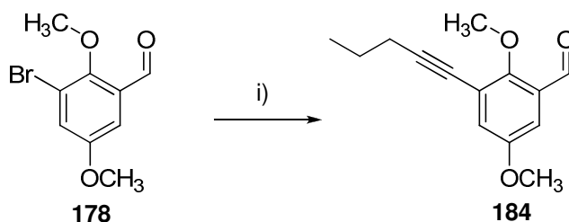
Scheme 2.13: Attempted Sonogashira coupling on 2,5-dimethoxy-3-bromobenzaldehyde 178
