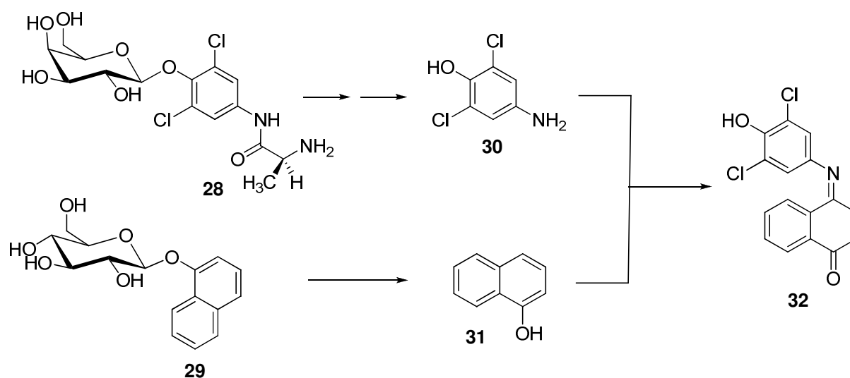
Scheme 1.9: Detection of three different enzyme activities: L-alanine-aminopeptidase and \beta -galactosidase activities to hydrolyse 28 and \beta -glucosidase activity to hydrolyse 29 .
