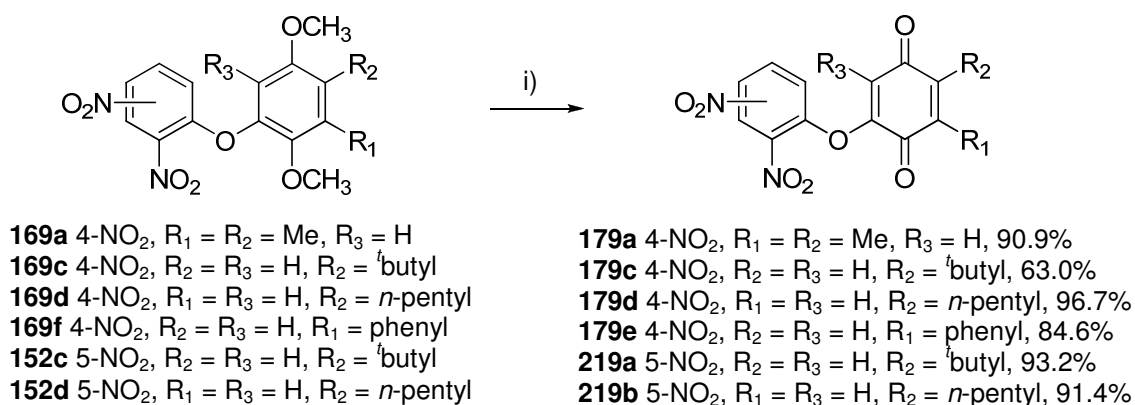
Scheme 2.38: Oxidative demethylation of substituted 2,4- and 2,5-dinitro-2',5'-dimethoxydiphenylethers i) CAN, CH 3 CN, H 2 O, R.T.
