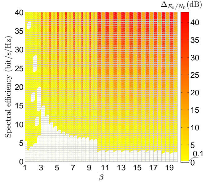
Fig. 4. Approximation error in terms of E_b/N_0 (dB) between the nearly-exact E_b/N_0 and the approximation method of [6] as a function of the SE and \bar{\beta} = \max\{t, r\} / \min\{t, r\} .
