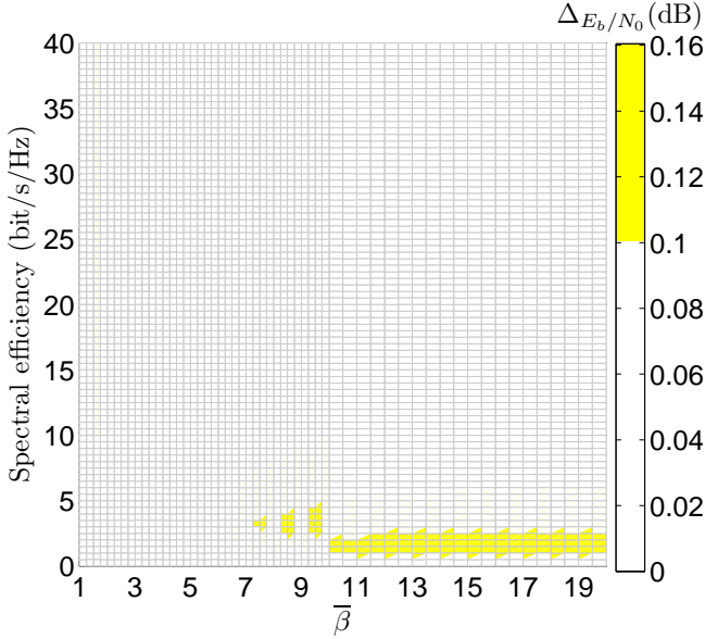
Fig. 3. Approximation error in terms of E_b/N_0 (dB) between the nearly-exact E_b/N_0 and our CFAs in (15) and (18) as a function of the SE and \bar{\beta} = \max\{t, r\} / \min\{t, r\} .
