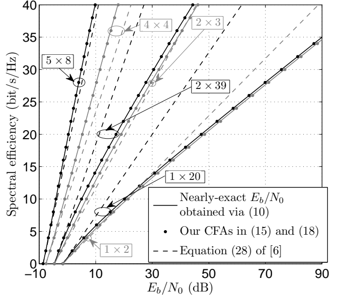
Fig. 5. Comparison of our EE-SE trade-off CFAs in (15) and (18) with the approximation method of [6] and the nearly-exact E_b/N_0 obtained via (10) for various r \times t antenna configurations.
