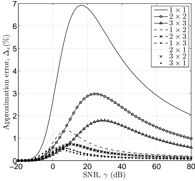
Fig. 1. Approximation error in % between \tilde{f}(\gamma) in (12) and f(\gamma) in (10) as a function of \gamma (dB) for various r \times t antenna configurations.
