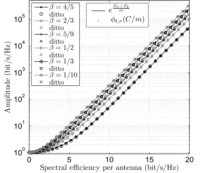
Fig. 2. Comparison of e^{\frac{S_r - S_t}{m}} with our parametric function \phi_{t,r}(C/m) as a function of the SE per antenna for various receive/transmit antenna ratios.
