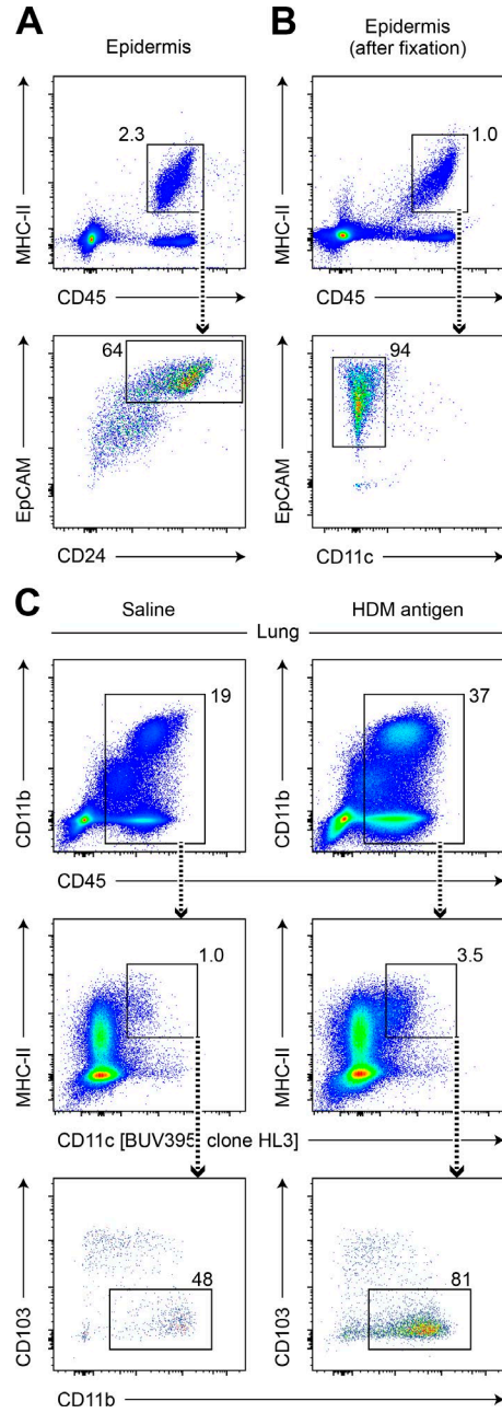
Figure S2. Gating strategies for the identification of LCs in the epidermis and monocyte-derived cells in the inflamed lung by flow cytometry. (A–C) After size and doublet discrimination using forward scatter and side scatter properties, samples isolated from the epidermis (A and B) or lung (C) were gated as indicated before further analysis in Fig. 4 and 5. Shown are representative two-color histograms; numbers indicate percentage of cells within the indicated gate.
