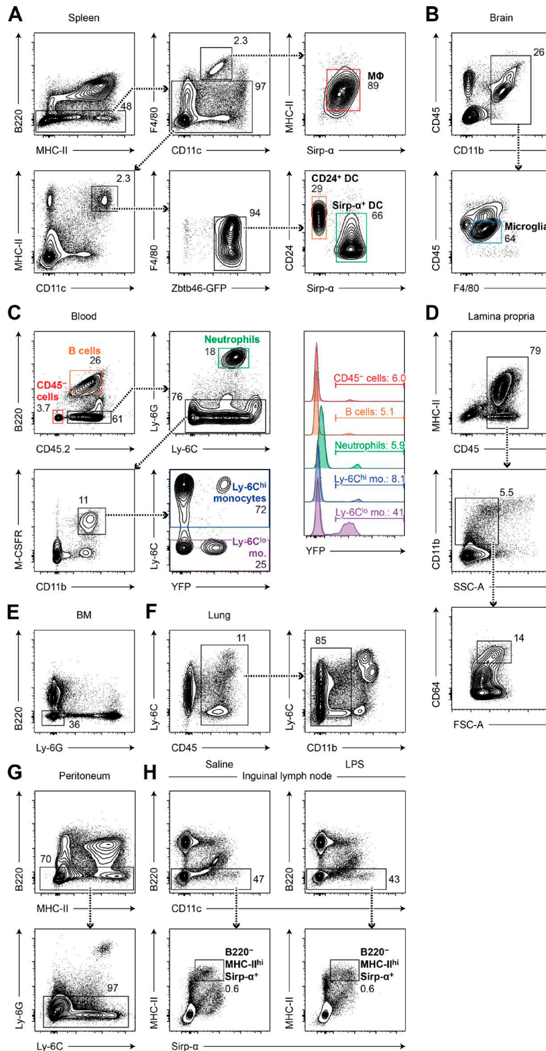
Figure S1. Gating strategies for the identification of monocytes, macrophages, and other populations by flow cytometry. (A–H) After size and doublet discrimination using forward scatter (FSC) and side scatter (SSC) properties, samples isolated from the spleen (A), brain (B), blood (C), lamina propria (D), BM (E), lung (F), peritoneum (G), or inguinal LN (H) were gated as indicated before further analysis in Fig. 2 and 3. Shown are representative two-color histograms; numbers indicate percentage of cells within the indicated gate. mo., monocytes; MΦ, macrophages.
