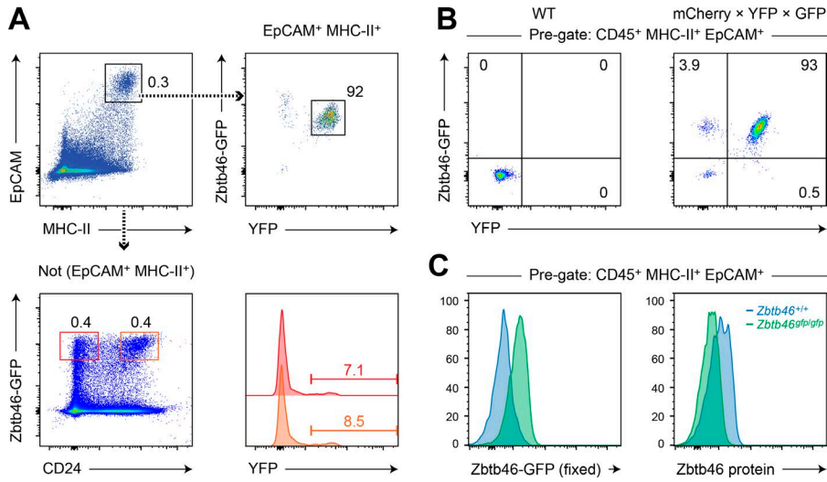
Figure 4. LCs at steady state are marked by MafB -driven lineage tracing but express Zbtb46 . (A) Migrated LCs in the inguinal LN of MafB -mCherry-Cre \times R26-stop-YFP \times Zbtb46 -GFP mice are displayed for expression of Zbtb46 -GFP and lineage-tracing marker YFP in a two-color histogram (top), and dermal DC populations in the same tissue identified by Zbtb46 -GFP and CD24 are displayed for expression of YFP (bottom). Shown is one representative sample ( n \geq 4 animals over at least two independent experiments). (B) LCs in the epidermis of wild-type or MafB -mCherry-Cre \times R26-stop-YFP \times Zbtb46 -GFP ( mCherry \times YFP \times GFP) mice, gated as in Fig. S2 A, are compared for expression of Zbtb46 -GFP and YFP in two-color histograms. Shown is one representative sample per group ( n \geq 2 animals per group over at least two independent experiments). (A and B) Numbers indicate percentage of cells within the indicated gate. (C) LCs in the epidermis of wild-type ( Zbtb46 +/+ ) or Zbtb46 -deficient ( Zbtb46 gfp/gfp ) mice, gated as in Fig. S2 B, are compared for expression of Zbtb46 -GFP and Zbtb46 protein in one-color histograms. Shown is one representative sample per group ( n = 3 animals per group over two independent experiments).
