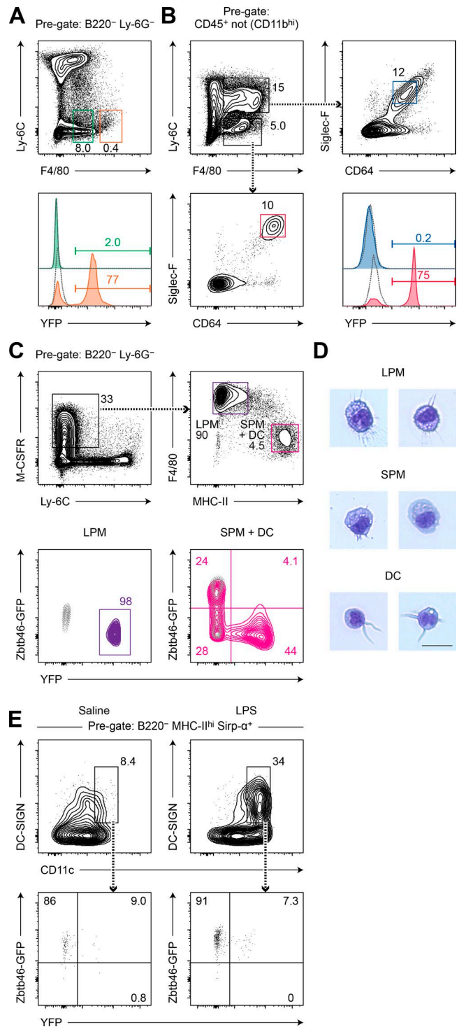
Figure 3. Mafb -driven lineage tracing segregates macrophages from other populations. (A) Macrophages in Mafb -mCherry- Cre × R26 -stop-YFP × Zbtb46 -GFP mouse BM, identified by surface markers as indicated (orange) after pre-gating as in Fig. S1 E, are compared with F4/80 + cells of similar immunophenotype (green) for expression of lineage-tracing marker YFP. Shown is one representative sample ( n \geq 4 animals over at least two independent experiments). (B) Alveolar macrophages in Mafb -mCherry- Cre × R26 -stop-YFP × Zbtb46 -GFP mouse lung, identified by surface markers
