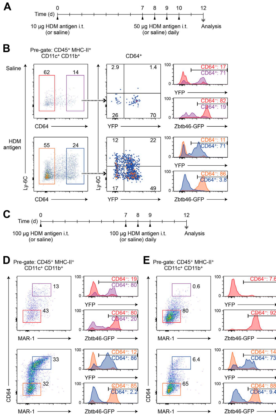
Figure 5. Ly-6C + monocyte-derived cells in the inflamed lung mature without expressing Zbtb46. (A) Experimental outline for intratracheal (i.t.) sensitization and challenge of MafB-mCherry-Cre × R26-stop-YFP × Zbtb46-GFP mice using HDM antigen. (B) Classical DCs and monocyte-derived cells in the lung, identified by surface markers as indicated after pre-gating as in Fig. S2 C, are compared for expression of Ly-6C, lineage-tracing marker YFP, and Zbtb46-GFP after treatment with vehicle (saline) or HDM antigen following the schedule outlined in A. Shown is one representative sample ( n \geq 4 HDM-treated animals over at least two independent experiments). Numbers indicate percentage of cells within the indicated gate. (C) Experimental outline for high-dose intratracheal sensitization and challenge of MafB-mCherry-Cre × R26-stop-YFP × Zbtb46-GFP mice using HDM antigen. (D and E) Classical DCs and monocyte-derived cells in the lung (D) or mediastinal LN (E), identified by surface markers as indicated, are compared for expression of YFP and Zbtb46-GFP after treatment with vehicle (saline) or HDM antigen following the schedule outlined in C. Shown is one representative sample ( n = 2 HDM-treated animals over two independent experiments). Numbers indicate percentage of cells within the indicated gate.
