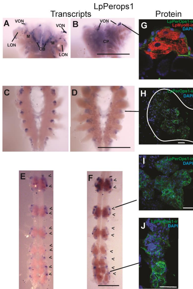
Figure 7. Distribution of LpPerOps1 transcripts and protein. LpPerOps1 transcripts and proteins were detected in the brain, synganglion and segmental ganglia of older juveniles. A-F. Representative whole-mount of the CNS from an older juvenile incubated with an antisense probe targeting LpPerOps1 transcripts. Dorsal views (A., C., F.) and ventral views (B., D., F) of the brain (A., B), synganglion (C., D.) and segmental ganglia (E., F). In the brain (A and B) LpPerOps1 transcripts were detected in the ventral optic nerve (VON), at the periphery of the lateral optic nerve (LON), in fibers that may be in the central body (CB), which is visible on the
