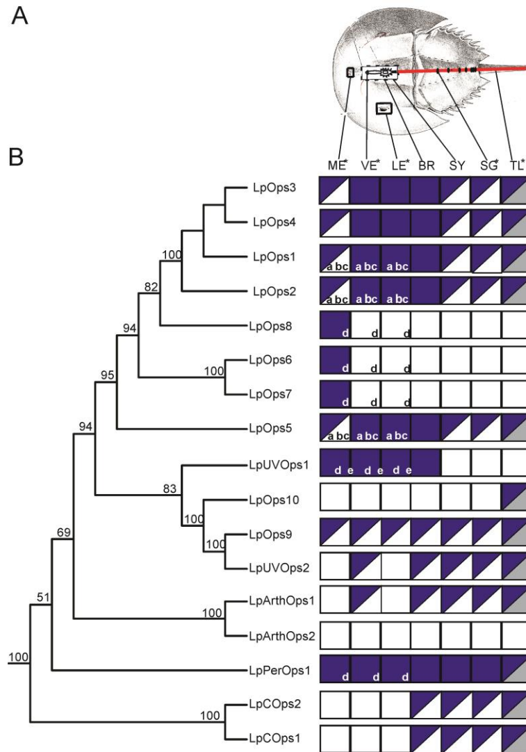
Figure 5. Distribution of opsin transcripts and protein in Limulus eyes and nervous system. A. Schematic of Limulus showing the locations of tissues tested for opsin transcripts by PCR and in situ hybridization and for opsin protein by immunocytochemistry. B. Left. Phylogenetic tree of Limulus opsins is modified from that shown in Figure 3. LpPerOps2 is not included here because transcripts encoding this opsin were not detected in any tissues assayed. LpArthOps2 is included because its transcripts were detected in the CNS of young juveniles. B. Right. Tissue distribution of the opsin shown at left. Top. Tissues assayed.
