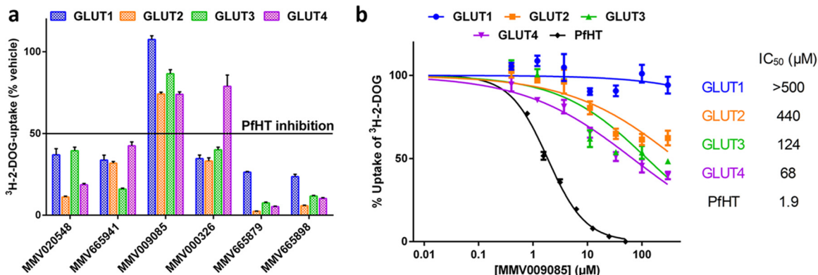
FIG 6 Specificity of hit compounds for PfHT over human orthologues. (a) Uptake of [ ^3\text{H} ]2-DOG by HEK293 cells overexpressing hGLUT1 to hGLUT4 in the presence of hit compounds at their \text{IC}_{50} for PfHT (Table 2). (b) Uptake of [ ^3\text{H} ]2-DOG by HEK293 cells overexpressing PfHT or hGLUT1 to hGLUT4 at increasing concentrations of compound MMV009085. Uptake data are expressed as means \pm SEMs ( n = 3 ). \text{IC}_{50} s were calculated using nonlinear regression analysis.
