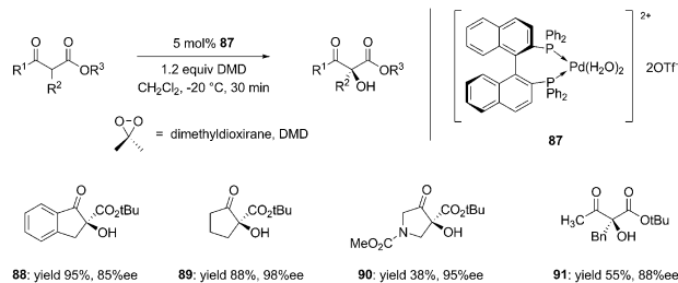
Scheme 22 Palladium-catalysed \alpha -hydroxylation of \beta -ketoesters with DMD as oxidant.
