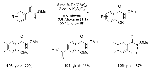
Scheme 25 Palladium-catalysed alkoxylation of aromatic C–H bonds.
