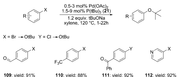
Scheme 27 Alkoxylation protocol established by Watanabe et al.
