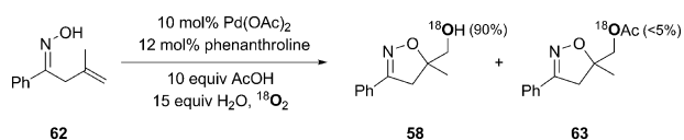
Scheme 15 Isotopic labelling experiments in the oxime-assisted intramolecular oxygenation of alkenes by palladium.
