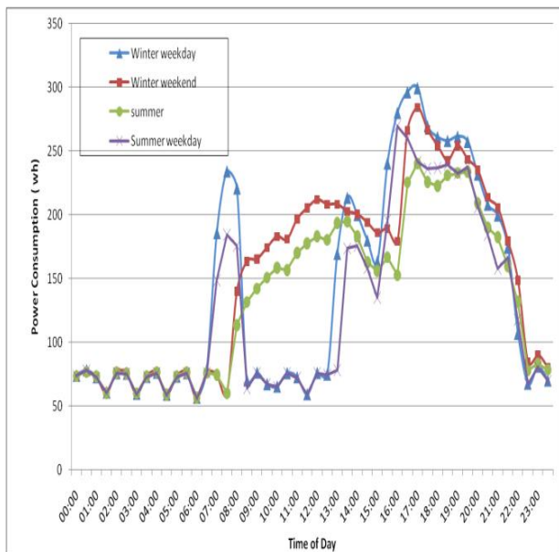
Figure 2. Daily winter and summer profiles.
