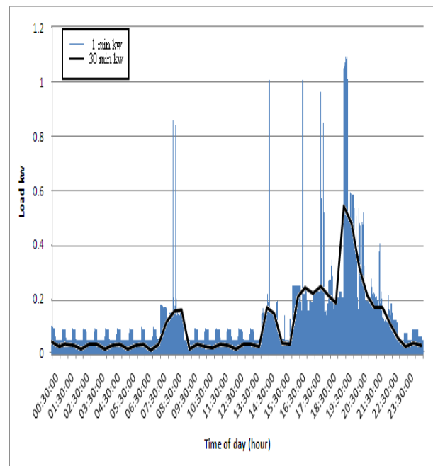
Figure 3. Daily load profile at 1 min and 30 min intervals
