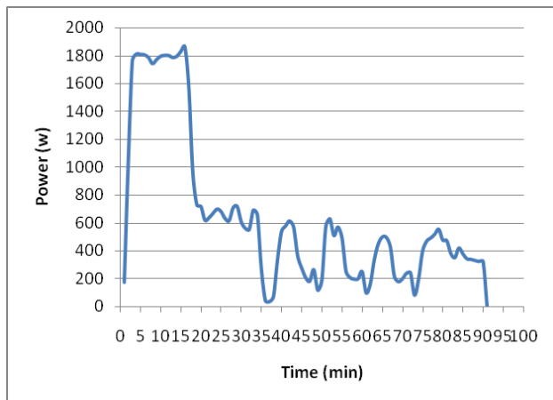
Figure 4. Washing machine electricity consumption profile
