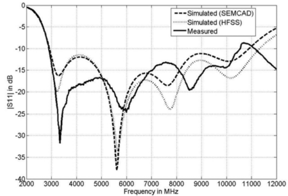
Figure 2 Measured and simulated reflection coefficients |S_{11}|
