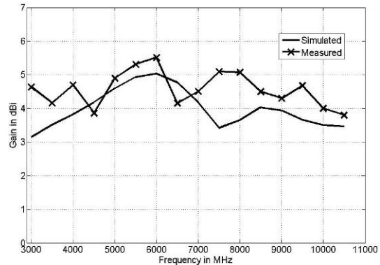
Figure 4 Measured and simulated antenna gains
