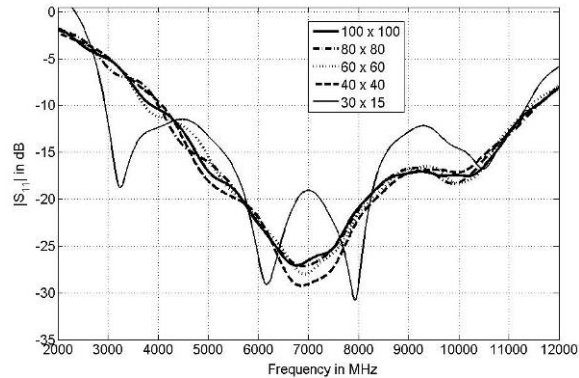
Figure 3 Simulated reflection coefficients |S_{11}| corresponding to the variation of ground plane size
