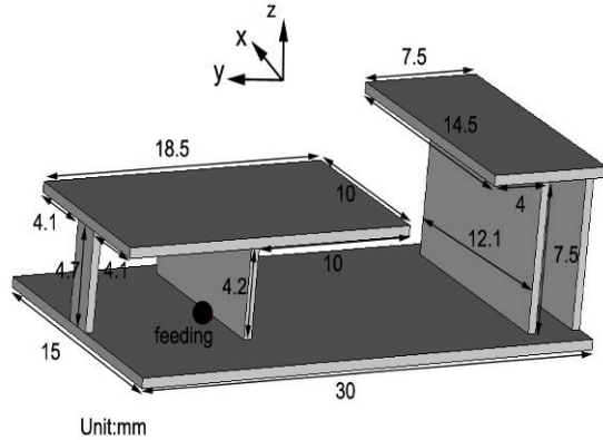
Figure 1 Geometry of the proposed antenna
