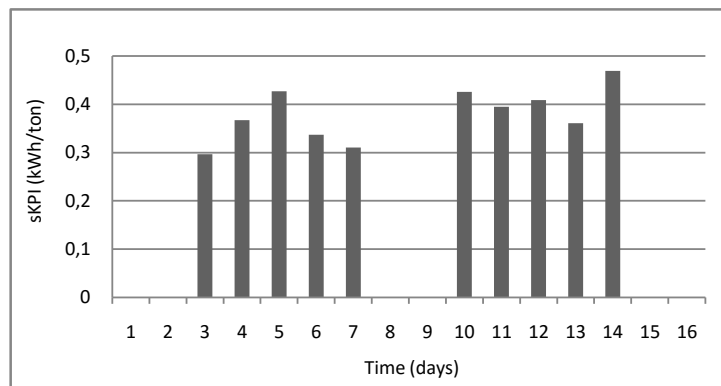
Fig. 3: Trend of sKPI (kWh/ton) in the reporting period.
