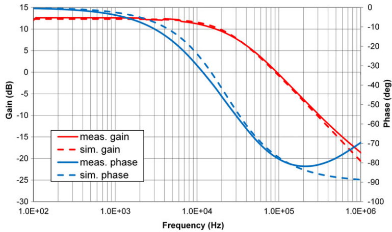
Figure 9. Bode plots of the differential gain (v_{out}^+ - v_{out}^-)/v_d magnitude and phase ( C_L = 40 pF): measured (solid lines) and simulated (dotted lines).
