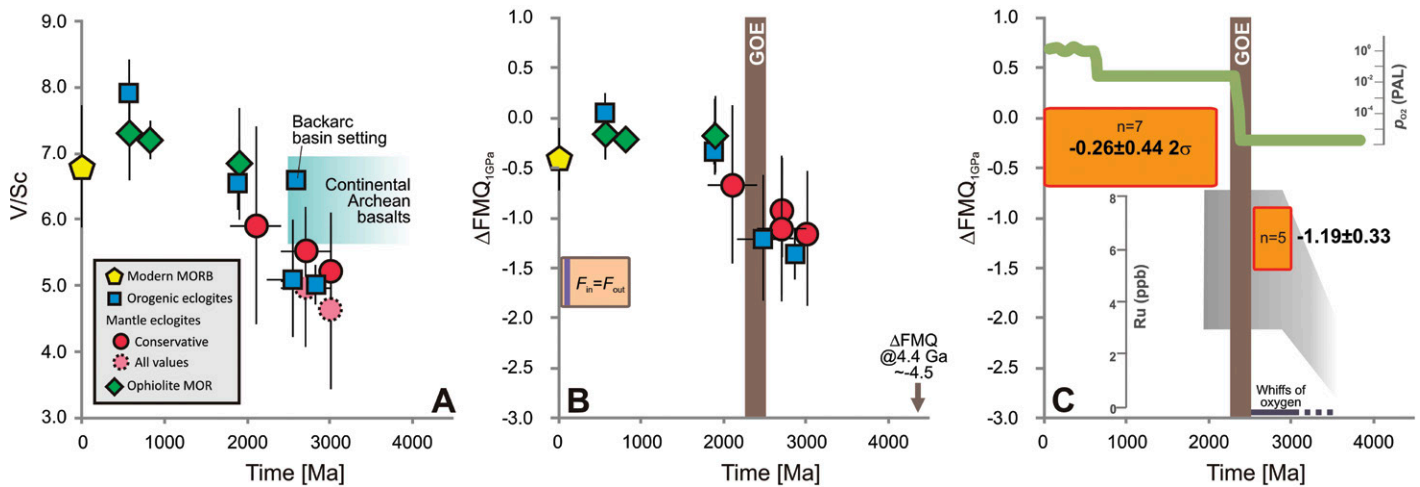
Figure 1. A: V/Sc of mid-ocean ridge (MOR)-derived metabasalts and basalts. MORB—mid-oceanic ridge basalt. B: Calculated oxygen fugacity ( f_{O_2} ) (relative to fayalite-magnetite-quartz buffer, \Delta FMQ ) corrected to 1 GPa. Error bars on V/Sc are 1\sigma of the mean per sample suite, those on \Delta FMQ are propagated 1\sigma errors of V/Sc, and those on the age are the cited 1\sigma errors for isochron-derived ages or age ranges reported in the literature. For two mantle eclogite suites (Victor [Superior craton, Canada] and Lace [Kaapvaal craton, South Africa]), two average values were calculated, where samples with the lowest V/Sc, of uncertain nature, were excluded for a conservative estimate. The range of V/Sc for continental Archean basalts is from Li and Lee (2004), and the estimate for convecting mantle immediately after core formation is from Frost and McCammon (2008). The timings of the Great Oxidation Event (GOE) and of the first “whiffs” of oxygen are from Lyons et al. (2014). F_{in} = F_{out} ( F —flux) corresponds to the crossover between volcanic gas compositions acting as oxygen sinks versus sources as a function of ambient mantle f_{O_2} (Holland, 2002; Li and Lee, 2004). C: \Delta FMQ (corrected to 1 GPa) averaged for all post-Archean sample suites (including modern MORB) and for all Archean sample suites. Boxes encompass mean \Delta FMQ \pm 2\sigma and age ranges for the sample suites. Gray field shows trend in Ru concentrations in mantle-derived komatiites (Maier et al., 2009); green line shows one possible evolution of atmospheric partial pressure of O_2 ( p_{O_2} ) relative to the present atmospheric level (PAL) (Lyons et al., 2014).
