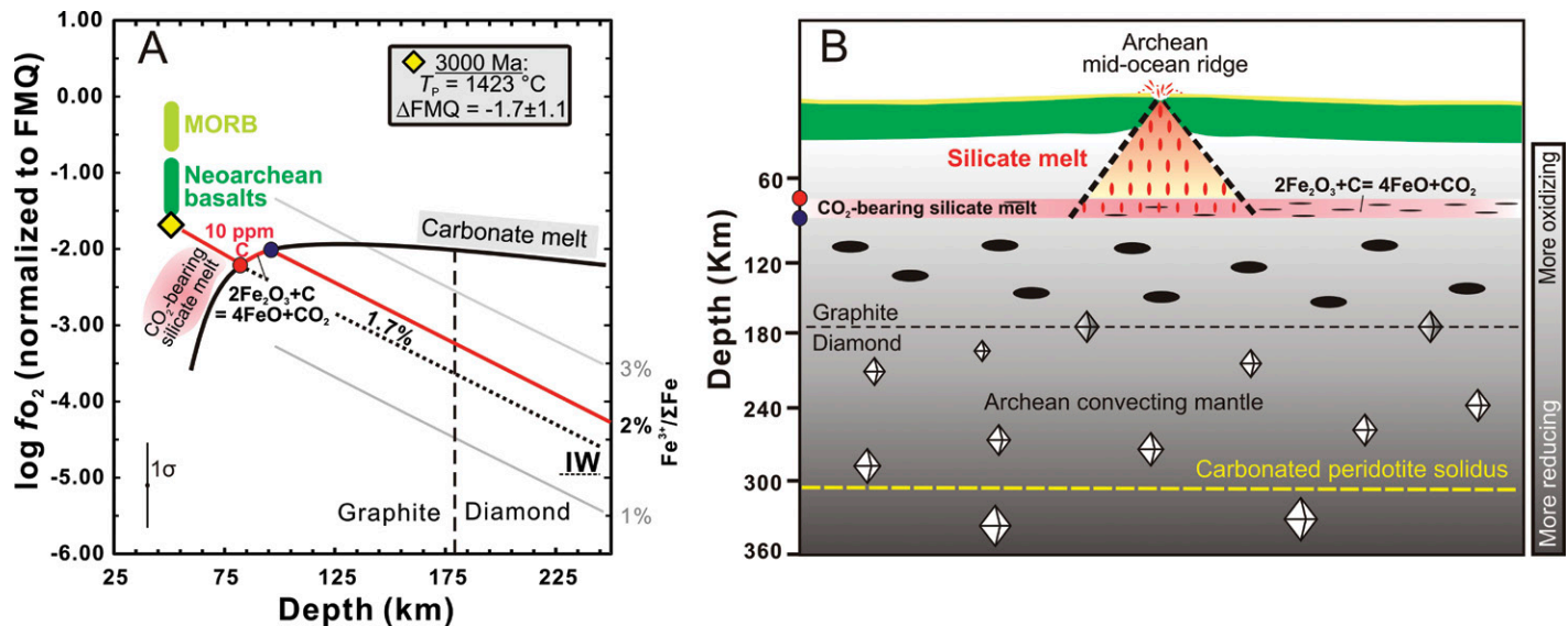
Figure 2. Speciation of carbon in the Archean mantle and origin of CO_2 -bearing melts. The composition of CO_2 melts results from the parameterization of oxygen fugacity ( f_{O_2} ) as functions of pressure ( P ), temperature ( T ), and X_{CO_2} . A: Mantle redox profiles ( f_{O_2} as a function of depth; gray lines) for different bulk rock Fe^{3+}/\Sigma Fe ratios (Stagno et al., 2013) at mantle potential temperature ( T_p ) of 1420^\circ C ; i.e., the temperature derived for the oldest mantle eclogite suite investigated here (3 Ga; Lace, Kaapvaal craton, South Africa; Aulbach and Viljoen, 2015). Calculations of f_{O_2} along an Archean mantle adiabat follow those of Stagno et al. (2013). Error bar shows 1\sigma on the oxy-thermobarometer employed. Black line indicates f_{O_2} at which graphite (or diamond) and carbonate melt (Stagno and Frost, 2010) coexist within a peridotite assemblage, calculated as function of P , T , and CO_2 content. With decreasing pressure during mantle upwelling, f_{O_2} drops owing to the increase in silica content in the melt. The ranges of f_{O_2} for mid-oceanic ridge basalt (MORB) and Archean basalts are from Lee et al. (2005) and this study, respectively. Mantle containing 2% Fe^{3+}/\Sigma Fe would be in the graphite stability field at depths <170 km. Redox melting [ C(\text{graphite}) + 2Fe_2O_3(\text{melt}) = 4FeO + CO_2 (both in the melt)] (Frost and McCammon, 2008) would occur in the depth interval of \sim 100 km (blue dot) and \sim 80 km (red dot) as the f_{O_2} of upwelling mantle crosses the equilibrium between graphite and carbonate-silicate melt ( CO_2 content \sim 10 wt%), with consequent reduction of Fe^{3+} in silicate phases (red line). The MORB f_{O_2} at 3000 Ma would result from oxidation of only 10 ppm of carbon in the depleted early mantle source (Dasgupta, 2013), which decreases the initial rock Fe^{3+}/\Sigma Fe ratio by <1\% . For higher carbon contents and lower T_p in the mantle source, silica-poor carbonated melts would be produced. The IW (iron-wustite) buffer is also indicated. B: Processes in the Archean convecting mantle as modeled in A (red line).
