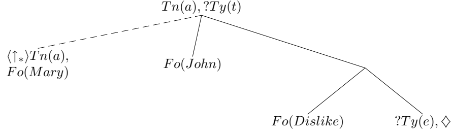
Figure 5: Parsing Mary, John dislikes
