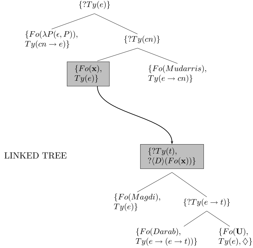
Figure 7: Parsing Il mudarris illi Magdi darab-u
