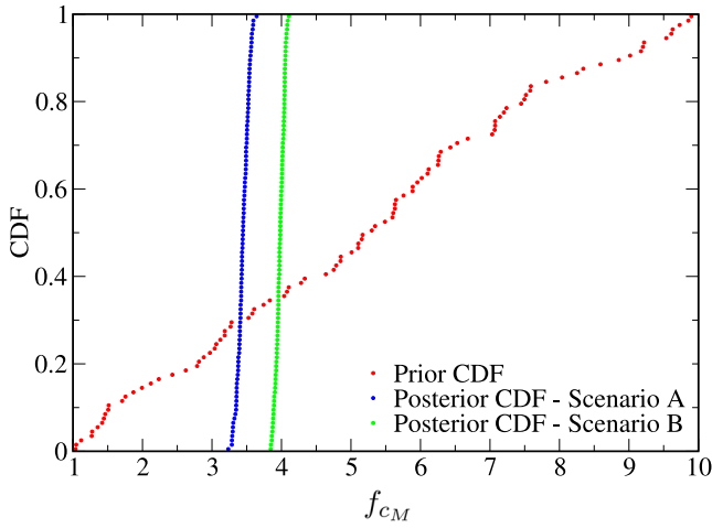
Figure 11. CM1: prior and posterior CDFs of the updating model parameter f_{c_M} for scenarios A and B.
