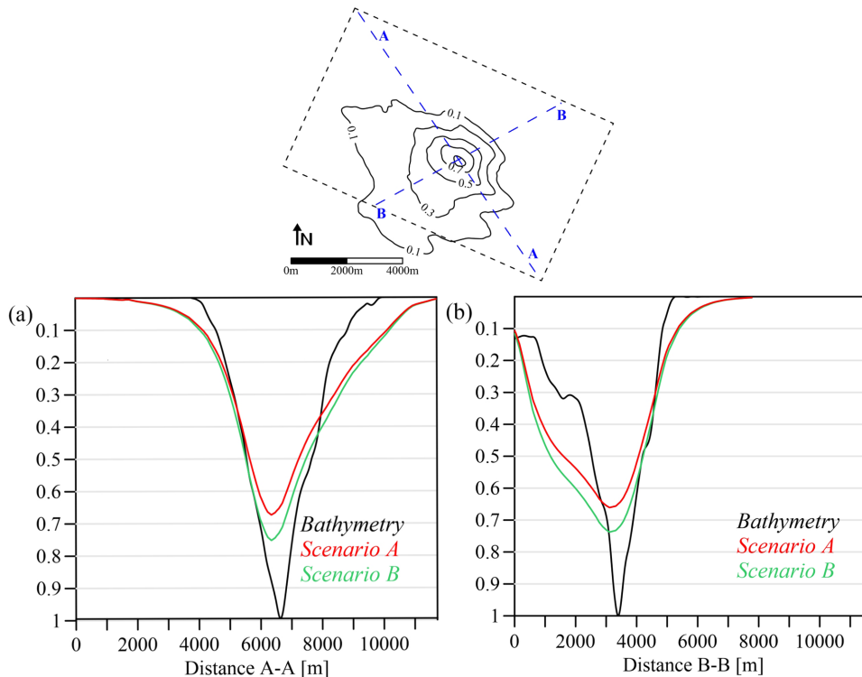
Figure 12. CM1: profiles of the mean seabed subsidence \mu_{v, \text{post}} along (a) section A–A and (b) section B–B traced on the top map. Scenarios A and B are compared with the bathymetric profile. Note that the subsidence values are normalized to u_{\text{max}} .
