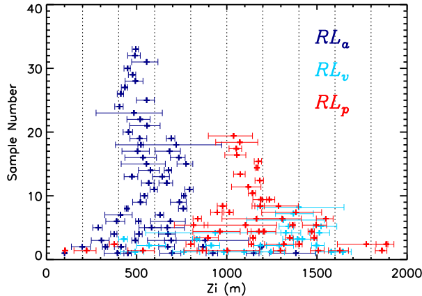
FIG. 10. The mean (+) and interquartile IQR range of z_{i,\text{ceil}} between 0000 LT and sunrise for each day color coded by RL class (absent, variable, and present). Frequency (y axis) is based on each day being classified based on the mean z_i into 200-m bins.
