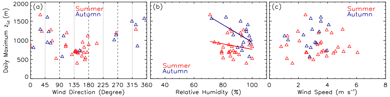
FIG. 12. Observed variation in summer and autumn daily maximum z_{i,c} and other variables measured at FX (based on ceilometer observations using S-IC) for RL_a cases as a function of (a) wind direction (at 10 m) at 0700 LT, (b) RH at 0700 LT (at 1.5 m) with linear regression lines to show the trend, and (c) mean wind speed between 0800 and 1200 LT.
