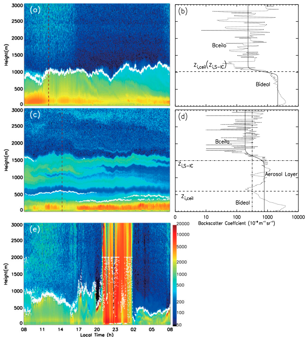
FIG. 3. Ceilometer backscatter coefficient and z_{i,\text{ceil}} (white diamond) for days that are (a) clear (24 h from 0800 LT 29 Dec 2013), (c) high aerosol (11 Sep 2013), and (e) rainy (24 h from 0800 LT 13 Sep 2013). (b),(d) Individual backscatter profiles (corresponding to vertical dotted red line in (a),(c), respectively) from one time (1319:44, 0133:08 LT, respectively) on each day and the fitted best ideal curve (vertical solid line) by Step-IC. Terms z_{i,S-IC} (horizontal dashed dotted line) and z_{i,\text{ceil}} (horizontal dashed line) are defined as the z_i directly retrieved by Step-IC and the one after aerosol examination process, respectively.
