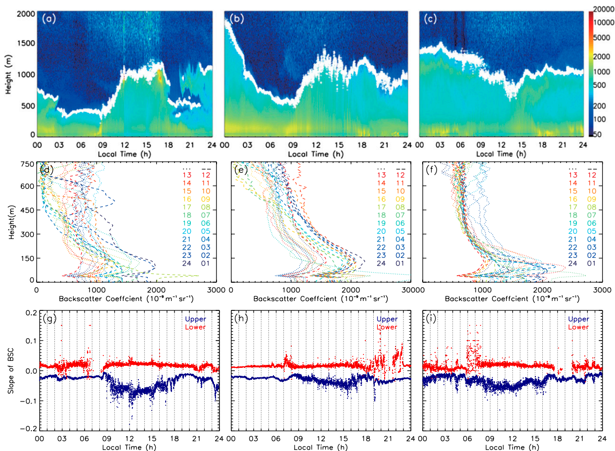
FIG. 9. Ceilometer backscatter coefficient \beta and z_{i,ceil} (white diamond) for examples of (a) residual layer absent RL_a (15 Feb 2014), (b) residual layer RL_v (28 Oct 2013), and (c) residual layer constantly present RL_p under clear skies (29 Nov 2013). Hourly (0100–2400 LT) \beta profiles between 0 and 750 m for (d) RL_a , (e) RL_v , and (f) RL_p , dashed and dotted lines are used for first and second halves of the day, respectively. Two heights with significant variation of \beta can be seen (sharp decrease SD around 40 m; inflection point IP around 130 m); time series of linear fit slopes between SD and IP ( S_{low} ) and the slope between IP and 300 m ( S_{up} ) for (g) RL_a , (h) RL_v , and (i) RL_p , respectively.
