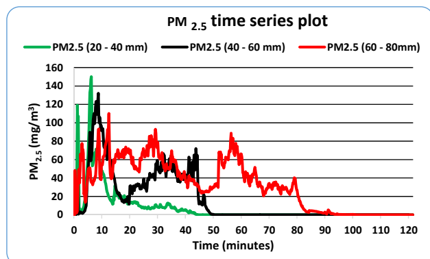
Figure 2: PM 2.5 time series plots for the three coal particle sizes in a high ventilation stove
