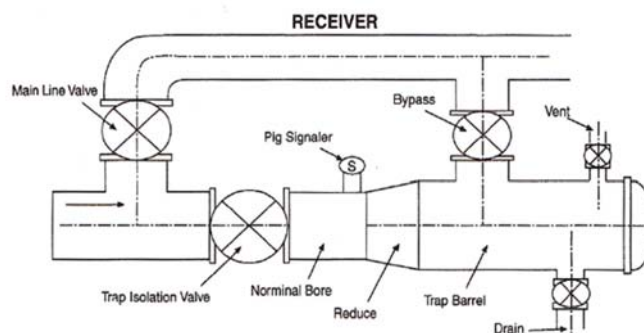
Figure 5. Typical pig receiver
