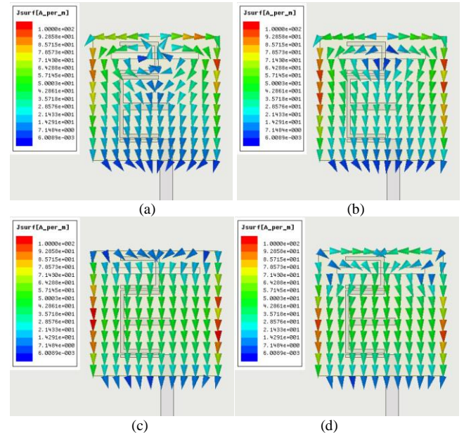
Fig. 8. The current distribution at the four operating frequencies: (a) 4.6 GHz, (b) 5.05 GHz, (c) 5.8 GHz and (d) 6.3 GHz.
