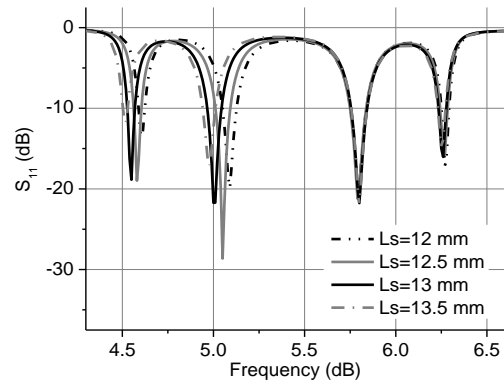
Fig. 6. The S_{11} of the four-band antenna with different L_s .
