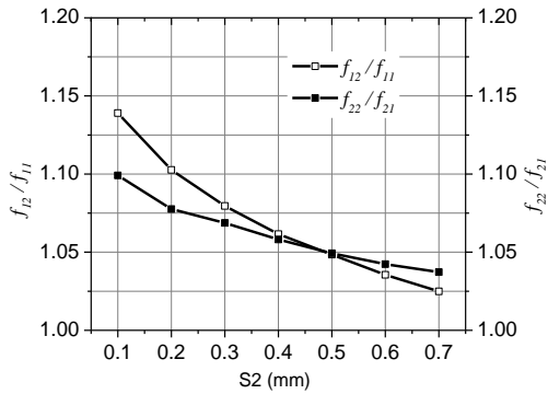
Fig. 5. The frequency ratios of f_{12}/f_{11} and f_{22}/f_{21} with different S2 .
