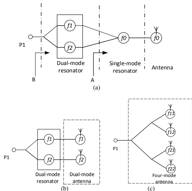
Fig. 1. The resonator-based topology: (a) topology of the proposed four-band antenna, (b) equivalent topology see from interface A, (c) equivalent topology see from interface B.
