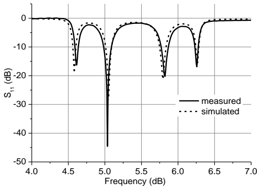
Fig. 9. The simulated and measured S_{11} of the proposed antenna.
