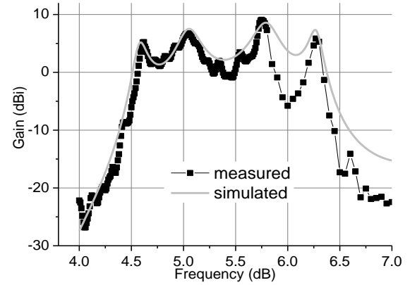
Fig. 11. The simulated and measured antenna gains.
