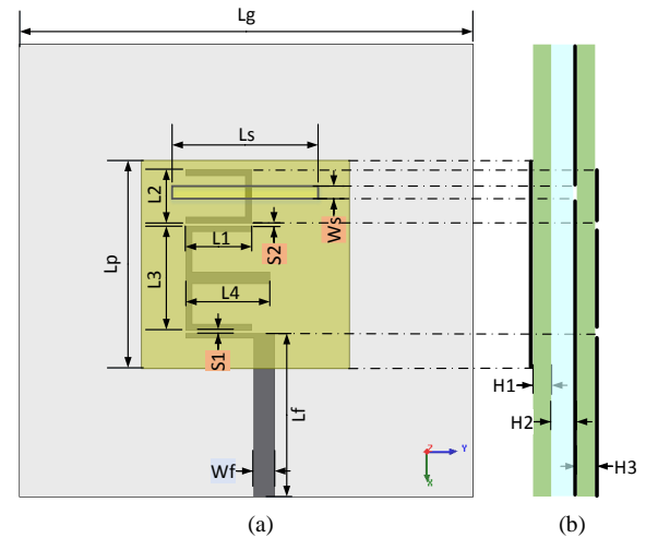
Fig. 2. Configuration of the proposed four-band patch antenna: (a) top view, (b) side view.
