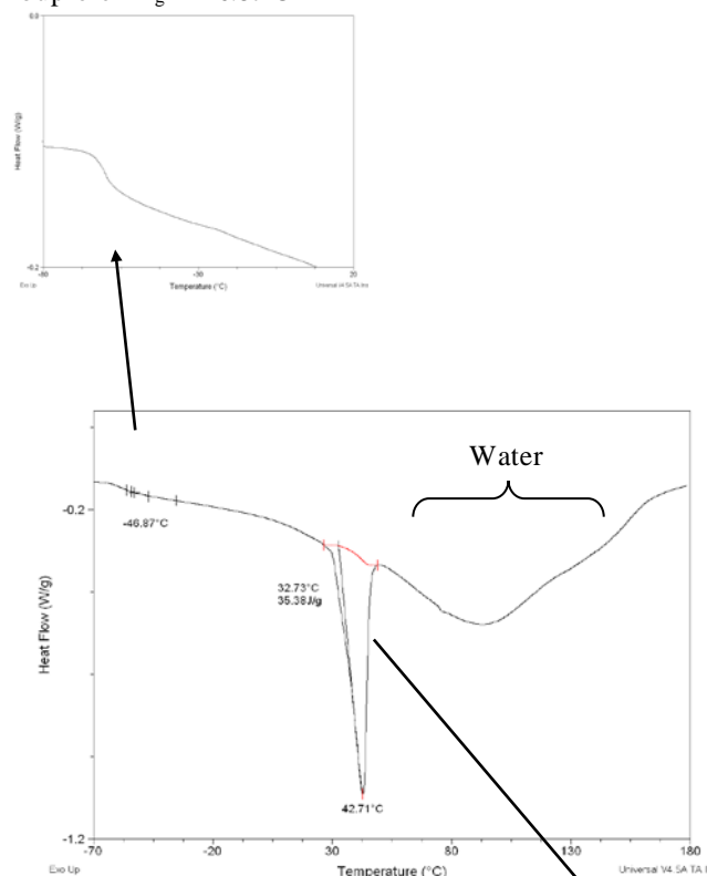
Fig. 1. DSC results for film containing ibuprofen. Poloxamer T_m = 42.7^\circ\text{C}
