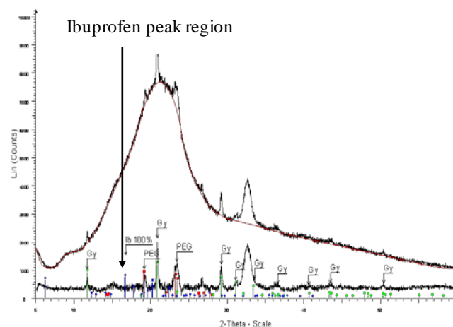
Fig.2. XRPD results for film containing ibuprofen.
