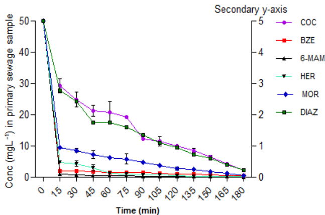
Figure 3: Plot showing combined concentrations of drugs in aqueous and solid phases in primary sewage sludge at 19 \pm 0.5^\circ\text{C} .
