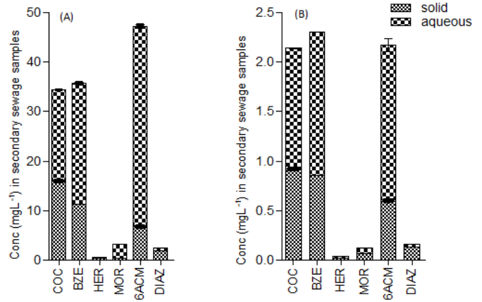
Figure 5: Degradation of compounds in SAF-1 sludge at time (A) 15 min and (B) 3h, demonstrating the change in distribution/partitioning as drugs degrade at 19 \pm 0.5^\circ\text{C} .
