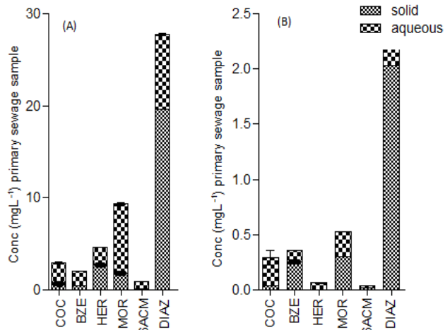
Figure 2: Degradation of compounds in primary sludge at time (A) 15 min and (B) 3h, demonstrating the change in distribution/partitioning as drugs degrade at 19 \pm 0.5^\circ\text{C} .
