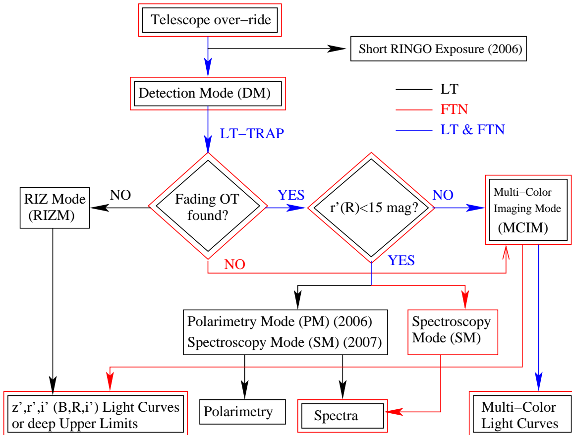
FIG. 2.— Diagram of the LT-TRAP observing strategy for both LT and FTN facilities.
