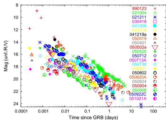
FIG. 1.— Early light curves (unfiltered, R and V ) for a set of GRBs with detections within minutes of the gamma-ray event. Big empty upside down triangles show the case of GRB 050502a (filter r' ) robotically detected and followed-up by LT (from Guidorzi et al. (2005a)). All the measurements shown have been taken from GCN circulars (Nos. 248, 257, 307, 715, 1572, 1589, 1596, 1732, 1738, 1739, 1748, 1752, 1759, 1821, 2773, 2776, 2784, 2798, 2799, 2821, 2875, 2897, 3118, 3165, 3480, 3485, 3487, 3489, 3492, 3575, 3584, 3588, 3596, 3601, 3604, 3646, 3704, 3705, 3711, 3712, 3716, 3717, 3718, 3720, 3723, 3726, 3728, 3733, 3736, 3739, 3741, 3744, 3745, 3746, 3756, 3765, 3775, 3778, 3829, 3834, 3836, 3838, 3853, 3863, 3864, 3865, 3868, 3869, 3870, 3880, 3883, 3896, 3907, 3917, 3929, 3943, 3944, 3945, 3947, 3950, 3953, 3960, 4011, 4012, 4015, 4016, 4018, 4023, 4026, 4027, 4032, 4041, 4044, 4046, 4048, 4049, 4095, 4120, 4121), except for GRB 030418 (Rykoff et al. 2004), GRB 041219a (Vestrand et al. 2005) and GRB 050502a (Guidorzi et al. 2005a).
