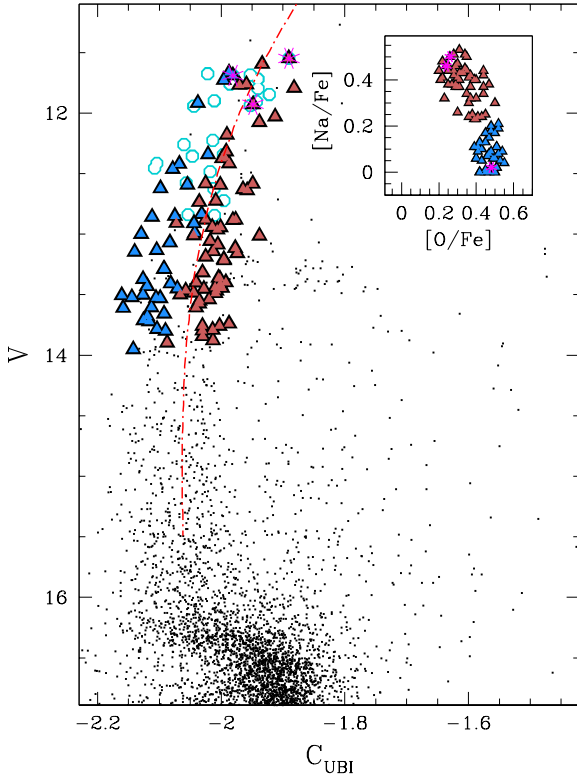
Figure 3. V - C_{UBI} diagram is shown. AGB stars and stars in common with the Marino et al. (2008) study are marked with the same symbols as in Figure 2. We display also a fiducial reference line (dash-dotted line) employed to quantify the broadening of the RGB and AGB sequences (see text for details). This line is just for reference, and is not meant to separate in this plot the location of FP and SP stars. The inset shows the NaO anti-correlation found by Marino et al. (2008) in M 4 RGB stars. FP and SP stars are plotted as blue and red triangles respectively in the V - \Delta C_{UBI} plane.
