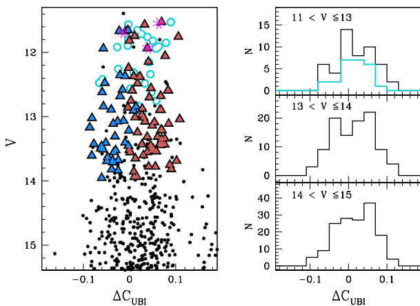
Figure 4. Verticalised V - \Delta C_{UBI} diagram for bright giant stars (see text for details). The number distribution of AGB (cyan histogram) and RGB (black histogram). \Delta C_{UBI} index differences with respect to the RGB fiducial in three V -magnitude bins are also shown. Magenta asterisks mark candidate AGB stars in common with Marino et al. (2008) .
