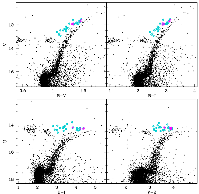
Figure 2. Selection of AGB star candidates in different CMDs. From top to bottom: V, B - V ; V, B - I ; U, U - I . Empty cyan symbols are AGB stars. Magenta asterisks mark candidate AGB stars in common with Marino et al. (2008) .
