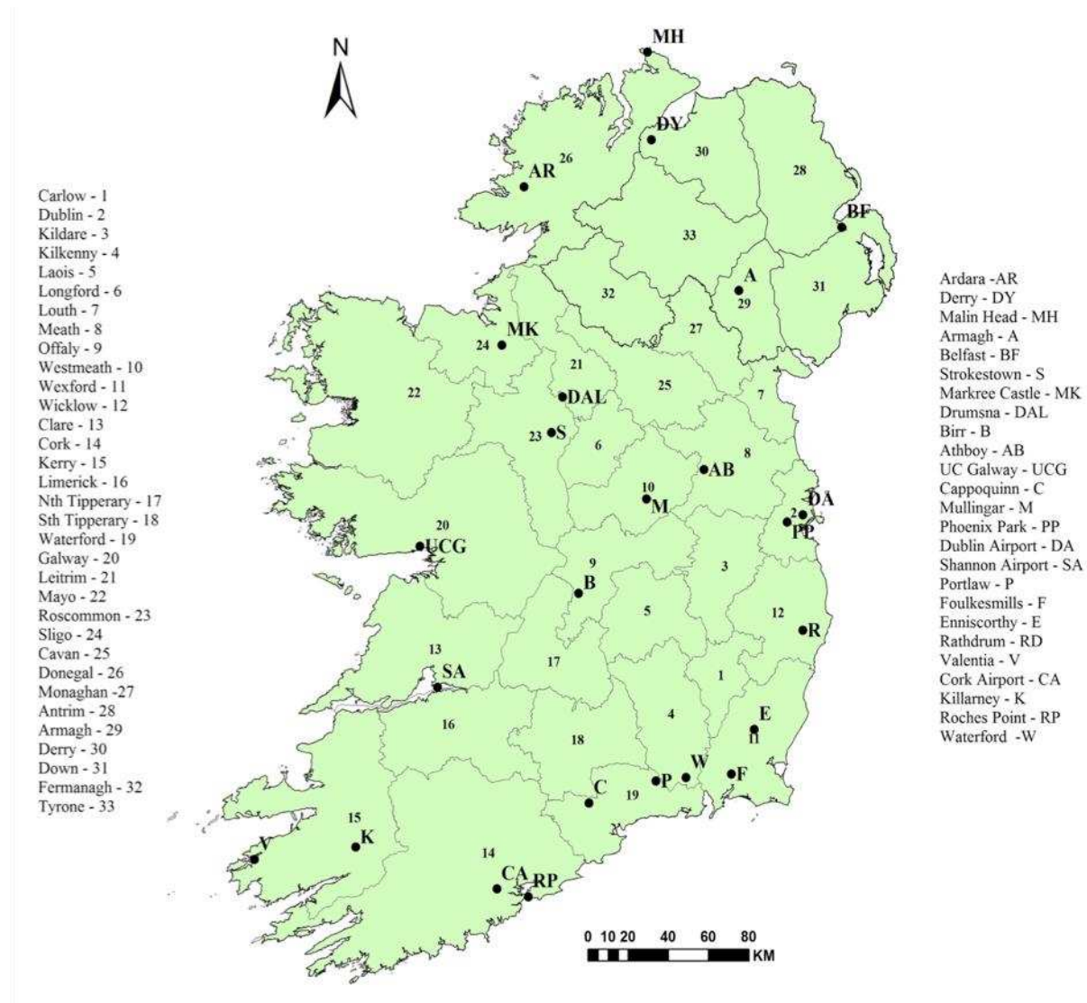
Figure 1. Location of the 25 stations in the Island of Ireland Precipitation (IIP) network and the abbreviated station names used in later figures. Also shown are counties of Ireland to provide context for documentary references to locations.
