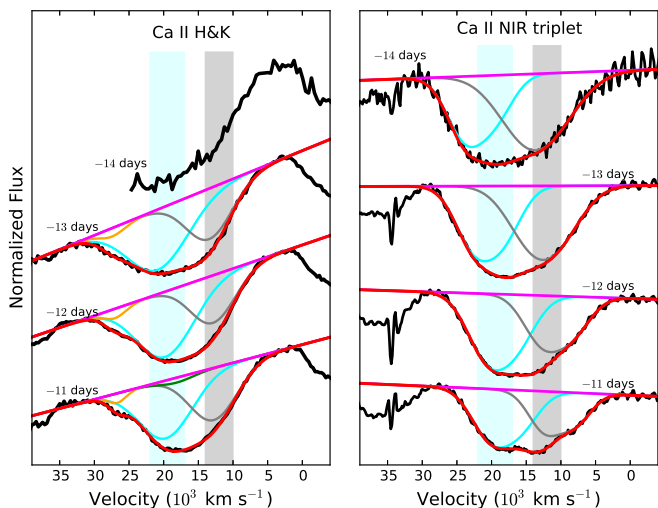
Figure 8. The spectral region around the Ca II H&K lines (left panel) and the NIR triplet (right panel) for SN 2015F at phases <-10 d. The magenta line corresponds to the pseudo-continuum, and the red profile is the resultant model from fitting Gaussian profiles to the observed spectrum. The profiles of the individual HV and photospheric components are shown in cyan and grey, respectively. In the left-panel the Si II \lambda 3856 line is shown in green, and the \sim 3600 Å feature in orange. The grey and cyan regions mark the positions of the photospheric ( 10000 – 14000 km s ^{-1} ) and HV ( 17000 – 22000 km s ^{-1} ) components.
