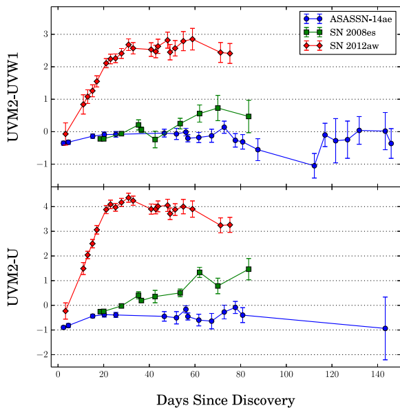
Figure 7. Comparison of (UVM2 - UVW1) (top panel) and (UVM2 - U) (bottom panel) color evolution between ASASSN-14ae (blue circles); SN 2008es, a super-luminous SN IIL (Gezari et al. 2009, green squares); and SN 2012aw, a SN IIP (Bayless et al. 2013, red diamonds). K-correction has been applied to the photometry for SN 2008es. ASASSN-14ae shows little evolution in either color while SN 2008es becomes redder in both colors and SN 2012aw becomes significantly redder over the first \sim 20 days after detection and remains roughly constant thereafter.
