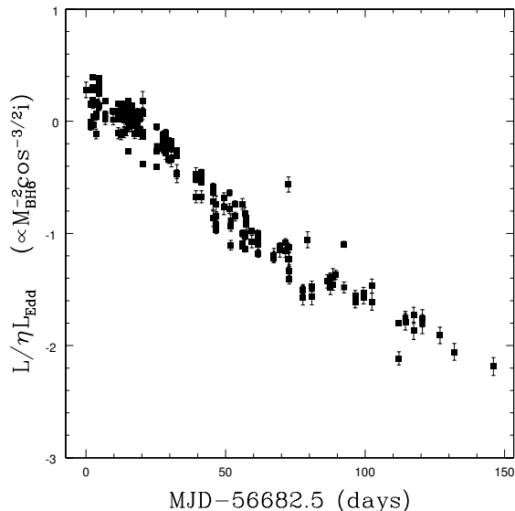
Figure 10. Implied luminosity in Eddington units of ASASSN-14ae using a thin disk model. The estimated L/L_{Edd} depends on the black hole mass M_{BH} = 10^6 M_{BH6} M_{\odot} , the disk inclination factor \cos i and the radiative efficiency \eta = 0.1\eta_{0.1} . Raising the black hole mass scale to M_{BH} \sim 10^{6.5} M_{\odot} would produce L/L_{Edd} \sim 1 at peak. In general, the SED of the thin disk fits the data significantly worse than a blackbody (see Figure 13 below).
