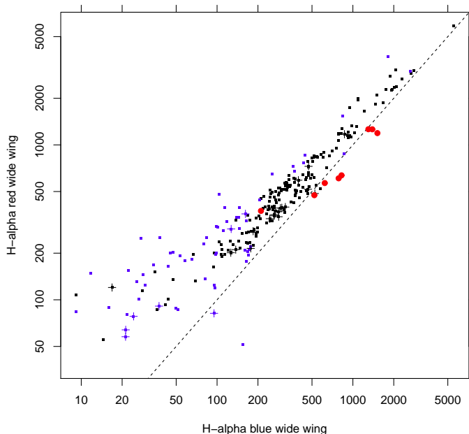
Fig. 20. Intensity of red vs. blue wide H\alpha wings. Datapoints from pure-sky fibres of HR15N (black) and HR14A (blue) setups. The dashed line is identity. The big red dots indicate the wide wings in the \eta Car spectra.
