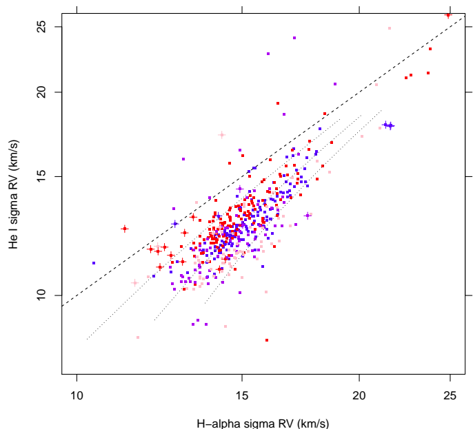
Fig. 9. Gaussian widths \sigma of He I lines vs. those of H\alpha . The three dotted lines represent loci of constant gas temperature, T_{gas} = 5000, 10000, 15000 K from top to bottom. The dashed line represents equality. Symbols as in Fig. 7. Only datapoints with the same RV from H\alpha and He I within 3 km/s are shown.
