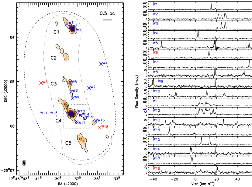
Figure 2. Detection of H 2 O masers and dense cores in the 20 km s -1 cloud (Lu et al. 2015). Left: The background image and the contours show the SMA 1.3 mm continuum emission, with levels between 5 \sigma and 65 \sigma in steps of 10 \sigma , where 1 \sigma =3 mJy beam -1 . The crosses show the H 2 O masers. The two red crosses (W6, W18) are masers with known OH/IR star counterparts. The dotted and green dashed loops show the FWHM of the SMA and VLA primary beams, respectively. Right: The spectra of the 18 H 2 O masers.
