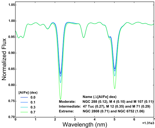
Figure 3. RSG models with solar-scaled (0.0 dex – as expected for the D15 RSGs) and enhanced ( >0.0 dex) [\text{Al}/\text{Fe}] values. We can exclude at high confidence that NGC 1705: 1 have extreme values of [\text{Al}/\text{Fe}] (like NGC 2808 or NGC 6752) that depart from the solar-scaled [\text{Al}/\text{Fe}] abundance of the RSGs from D15, cf. Fig. 2.
