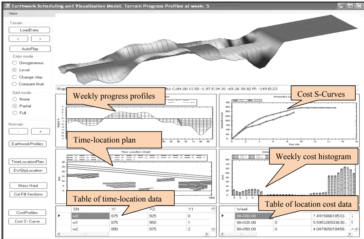
Fig 2 Snapshot of the visual outputs of model showing the location-based scheduling information
