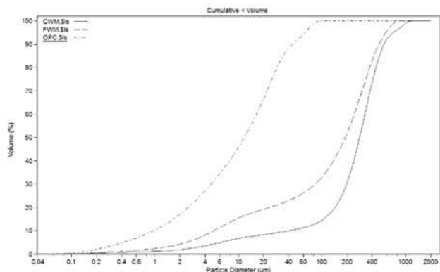
Fig. 3 Particle Size Distribution of the Waste Material Compared with OPC
