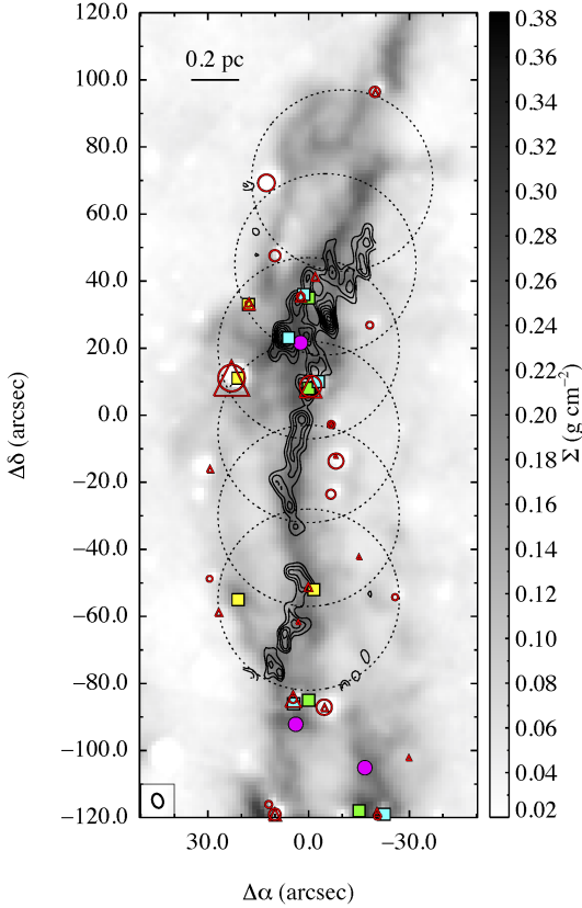
Figure 1. The combined mid- and near-infrared extinction-derived mass surface density map of Kainulainen & Tan (2013) (grey scale) overlaid with 3.2 mm continuum contours. Contour levels start at 3\sigma_{\text{rms}} and increase in steps of 2\sigma_{\text{rms}} (where \sigma_{\text{rms}} \approx 0.07 \text{ mJy beam}^{-1} ). Large dotted circles indicate the 6-field mosaic obtained with the Plateau de Bure Interferometer. Filled magenta circles indicate the locations of high-mass cores reported by Butler & Tan (2012). Filled cyan and yellow squares refer to the high-mass ( > 20M_{\odot} ) and low-mass ( < 20M_{\odot} ) dense cores identified by Nguyen Luong et al. (2011) from Herschel observations. Open red circles and red triangles refer to the 8 \mu\text{m} , and 24 \mu\text{m} emission, respectively (Carey et al. 2009; Jiménez-Serra et al. 2010). The symbol sizes are scaled by the source flux. Filled green squares highlight the location of extended 4.5 \mu\text{m} emission (Chambers et al. 2009).
