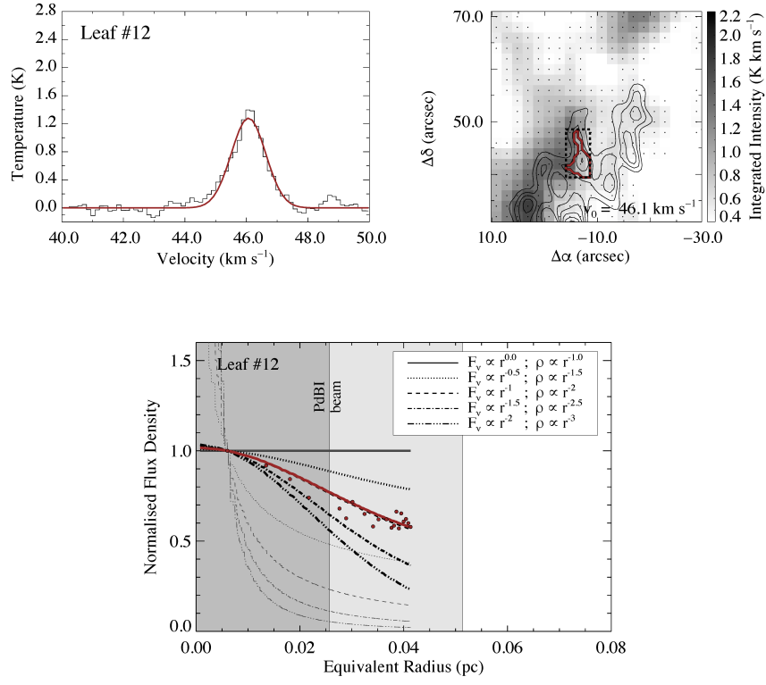
Figure A10. The average spectrum, spatial distribution of integrated \text{N}_2\text{H}^+ (1-0) emission, and the radial flux density profile of leaf #12.
