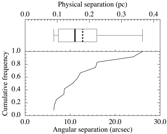
Figure 4. (Top) A box plot of the angular leaf separation. This highlights the range in separation, the interquartile range (the box itself), the median separation ( \sim 11.1 arcsec; thick vertical line), and the mean separation ( \sim 12.8 arcsec; vertical dashed line). (Bottom) The corresponding cumulative distribution.
