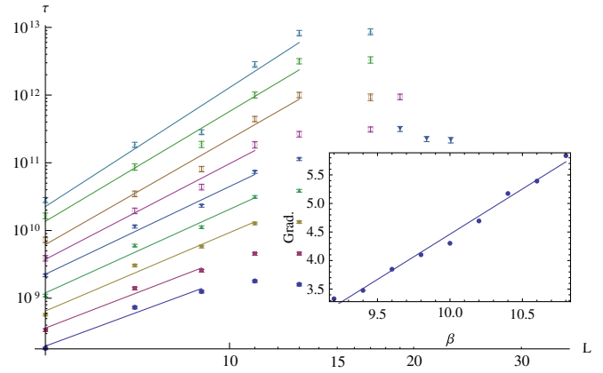
FIG. 15. Numerically evaluated coherence times \tau for the cubic code shown as a function of system size L . We show separate lines for \beta = 9.2, 9.4, \dots, 10.8 , where \beta = 9.2 is shown by the lower dark blue line and \beta = 10.8 is shown by the light blue line at the top. The inset shows the gradients of each of the lines in the main figure which, in this temperature regime, grow like \tau \sim L^{1.58\beta - 11.38} .
