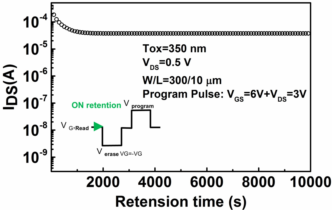
Fig S2: Decay of channel conductance measured at V_{DS}=0.5\text{V} and V_{GS, \text{Read}} = 0\text{V} after the application of a simultaneous gate (6V) and drain pulse (3V) for 5s shows a permanent retention behavior for a 350 nm oxide. The retention data is measured using the single pulse scheme shown in the inset of the figure.
