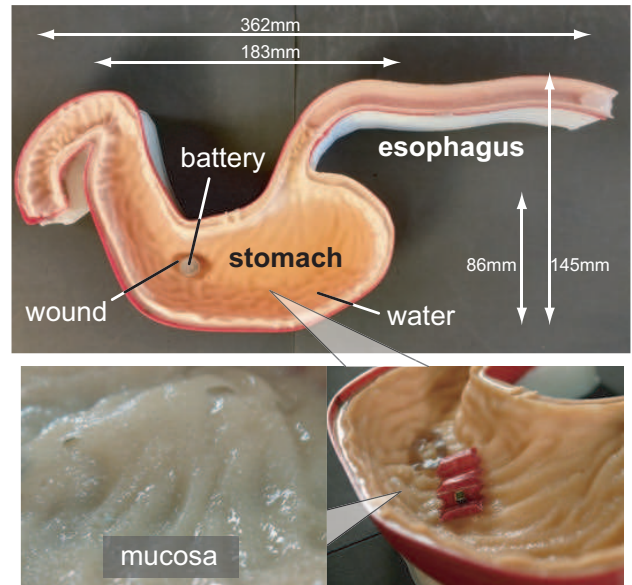
Fig. 2. Developed artificial esophagus and stomach (top) and details of the artificial mucosa (bottom).
